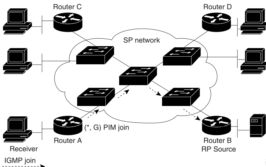
Figure 31-2 PIM Join Message Flow with PIM Snooping
