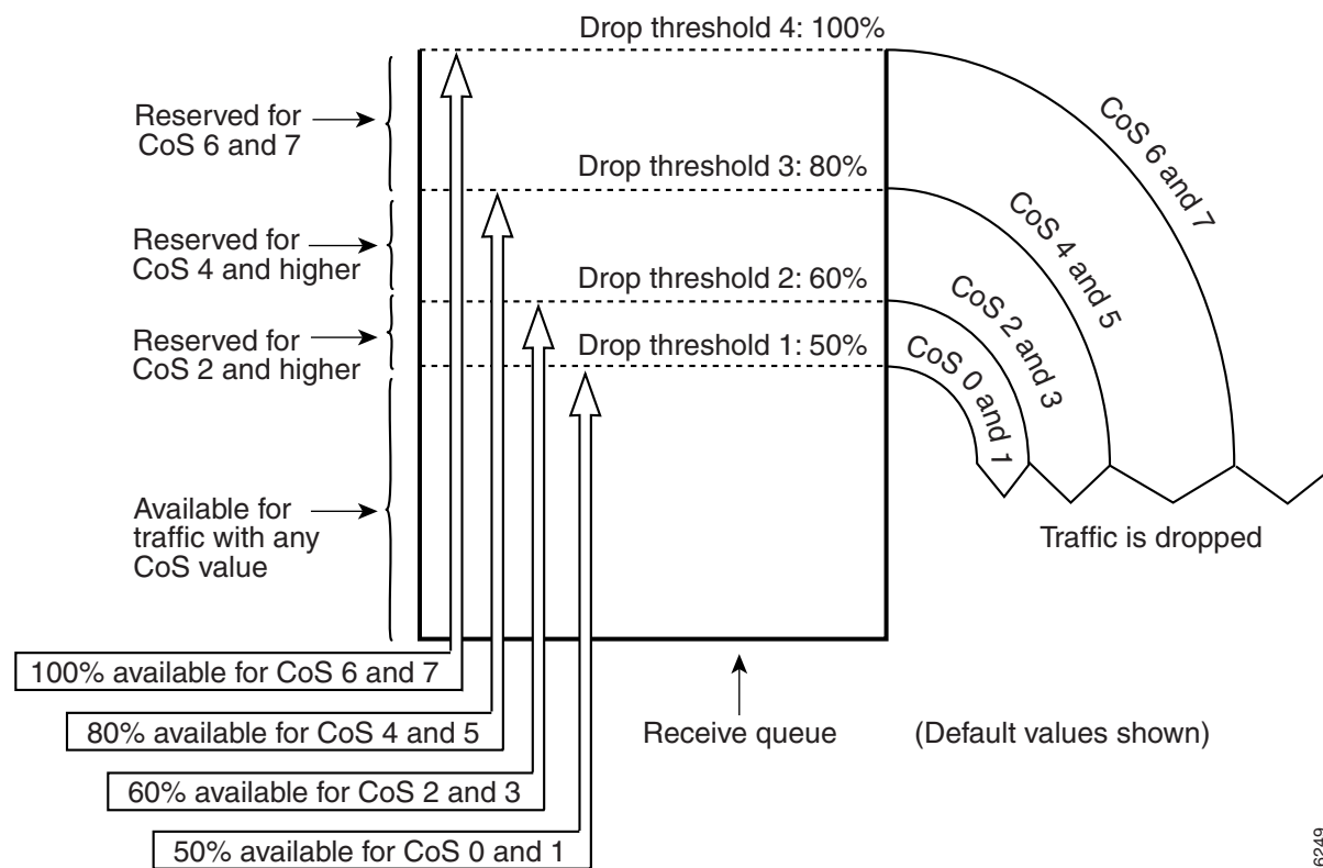
Figure 41-9 Receive Queue Drop Thresholds
