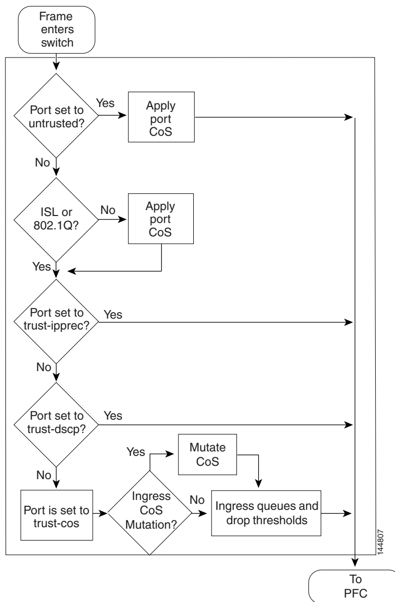
Figure 41-4 Ingress Port QoS Features
