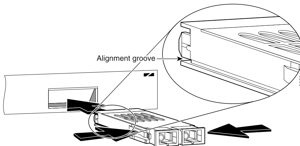
Figure 8 Inserting a GBIC Module with Alignment Groove on the Bottom
