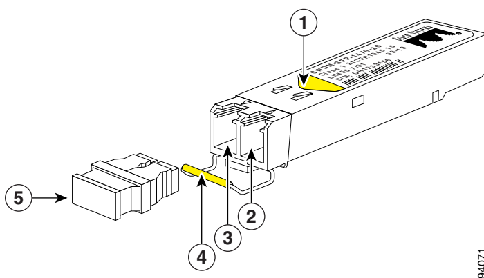
Figure 4 CWDM SFP Module
