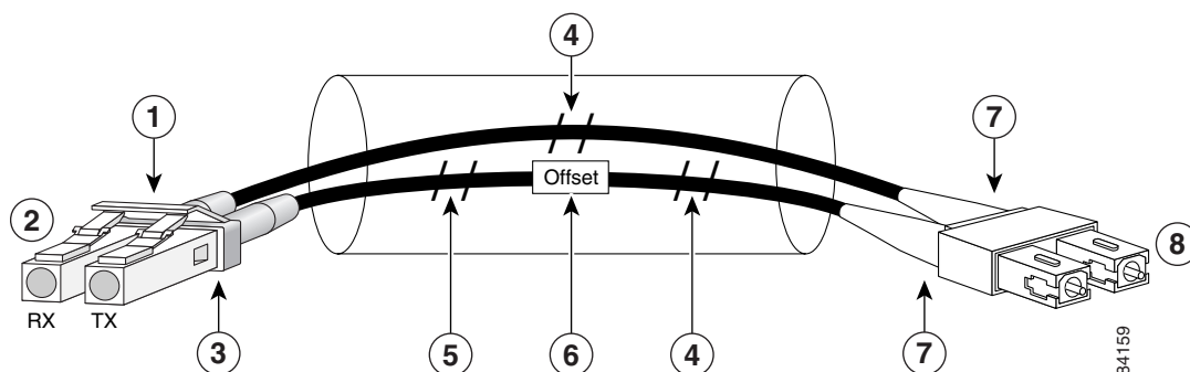
Figure 6 Mode Conditioning Patch Cord Assembly with SFP Module-Type Connector
