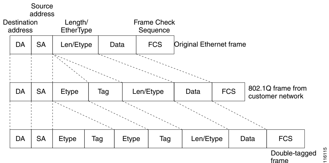
Figure 2 Untagged, 802.1Q-Tagged, and Double-Tagged Ethernet Frames
