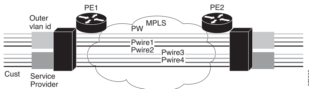
Figure 18-4 QinQ Connection
