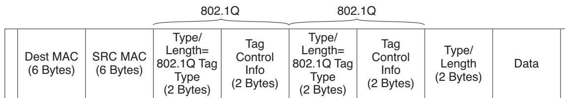
Figure 18-3 Ethernet VLAN QinQ Header
