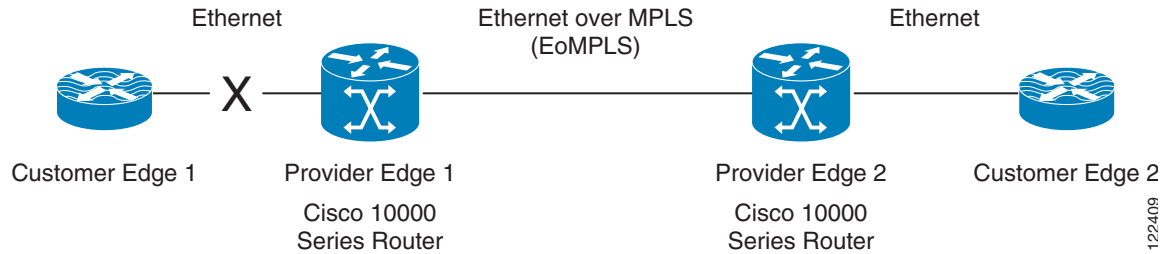
Figure 18-5 Remote Link Outage in EoMPLS Wide Area Network
