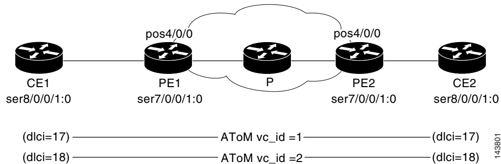
Figure 18-7 Frame Relay over MPLS Example Topology
