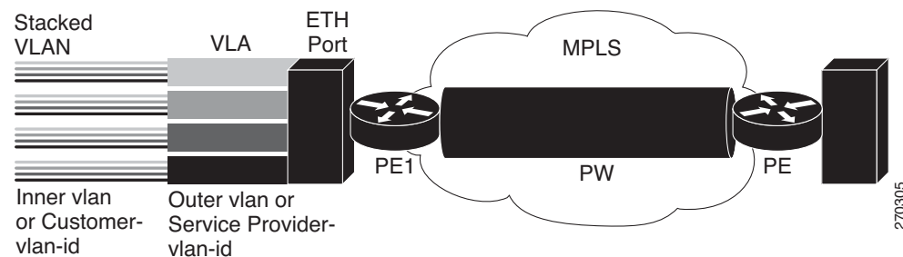
Figure 18-2 Ethernet VLAN QinQ
