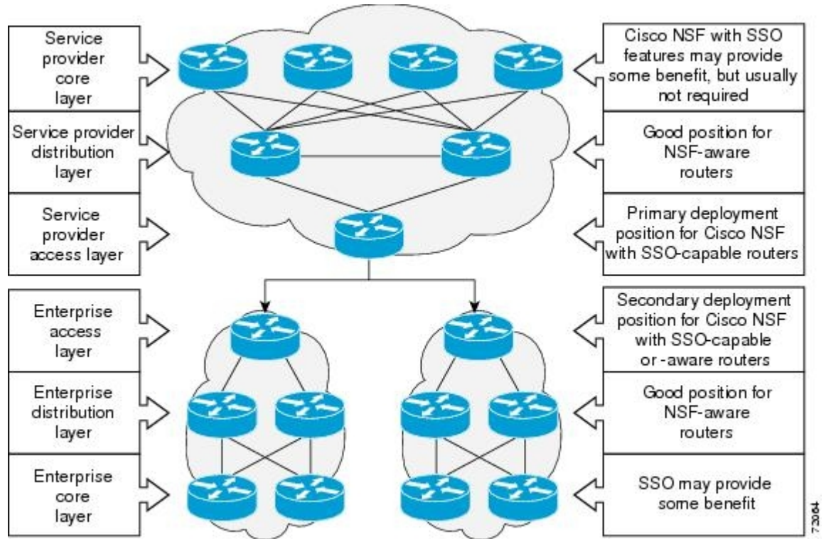
Figure 61: NSF with SSO Network Deployment: Enterprise Networks
