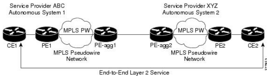
Figure 56: L2VPN Pseudowire Stitching in an Inter-AS Topology
