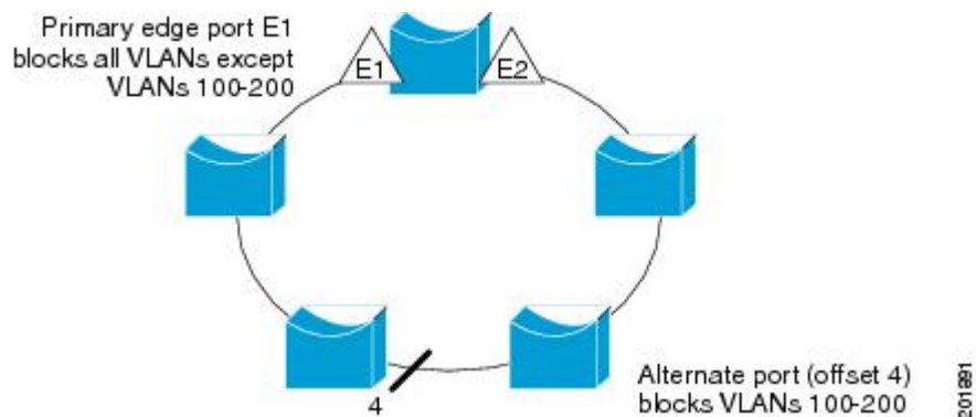
Figure 65: Example of VLAN Blocking
