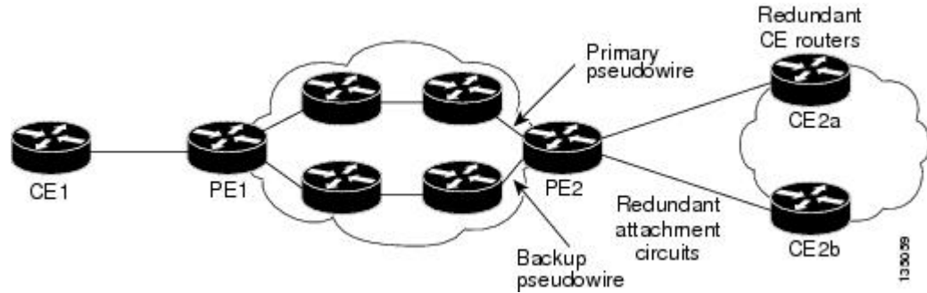
Figure 53: L2VPN Network with Redundant PWs, Attachment Circuits, and CE Routers
