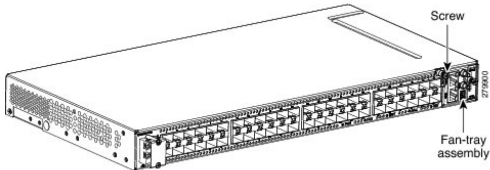
Figure 21: Fan-Tray Assembly in the CPT-50 Shelf
