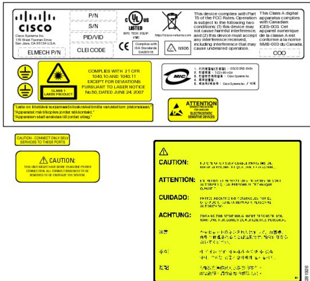
Figure 10: CPT 50 Shelf Label
