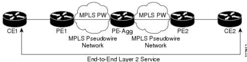
Figure 56: L2VPN Pseudowire Stitching in an Inter-AS Topology
