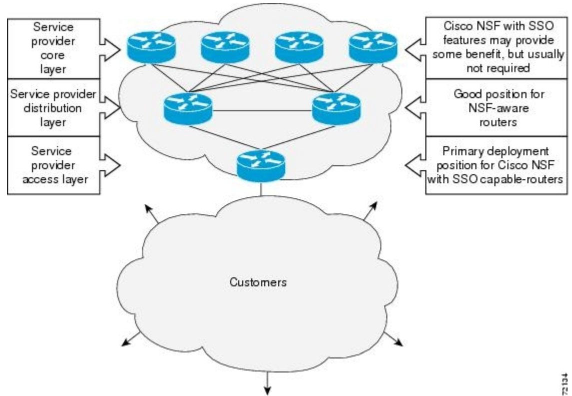
Figure 60: NSF with SSO Network Deployment: Service Provider Networks
