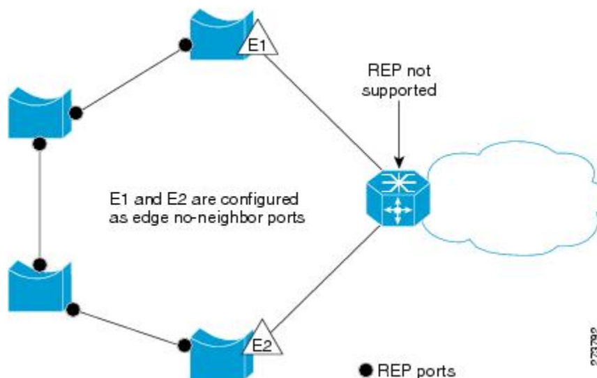
Figure 64: Edge No-Neighbor Ports
