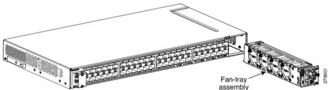
Figure 22: Fan-Tray Extracted
