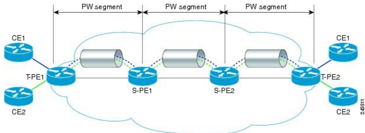
Figure 50: A Multisegment Pseudowire
