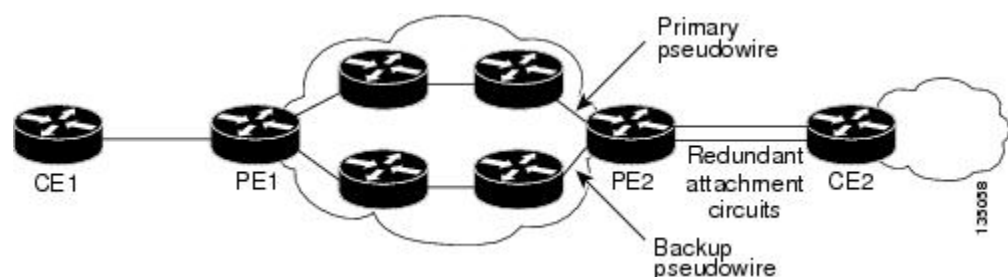
Figure 52: L2VPN Network with Redundant PWs and Attachment Circuits
