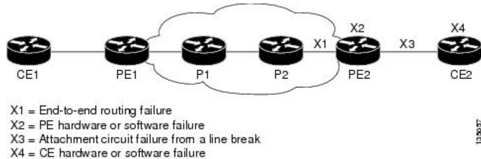
Figure 51: Points of Potential Failure in an L2VPN Network
