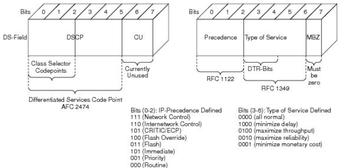
Figure 57: IP Precedence and DSCP
