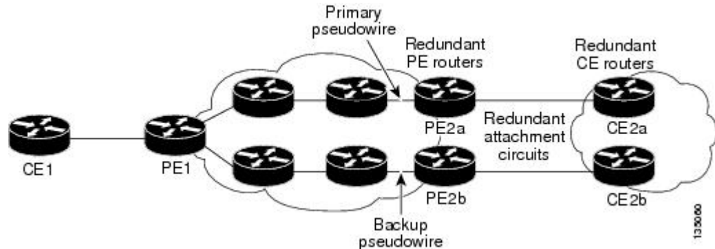
Figure 54: L2VPN Network with Redundant PWs, Attachment Circuits, CE Routers, and PE Routers
