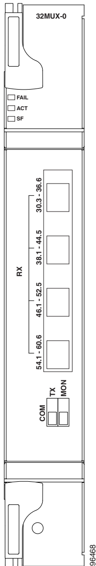
Figure 5-13 32MUX-O Faceplate
