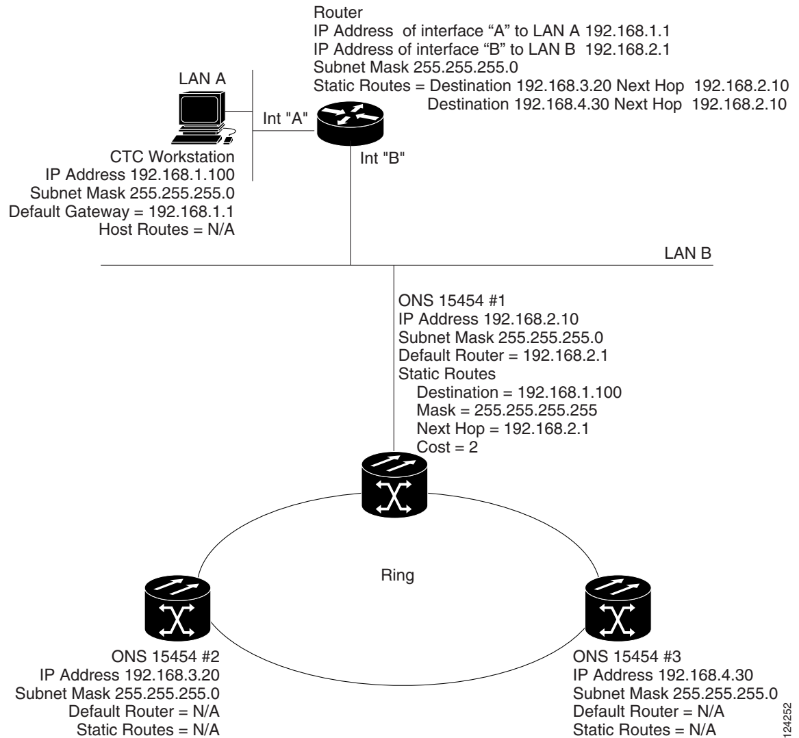
Figure 17-9 Scenario 6: OSPF Not Enabled (ANSI and ETSI)
