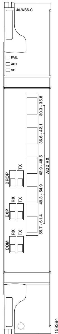
Figure 9-28 40-WSS-C Faceplate
