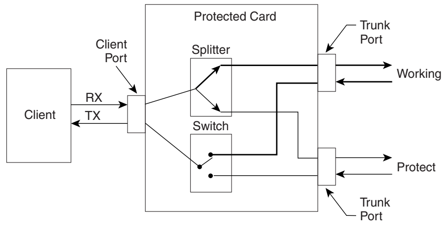
Figure 10-39 Splitter Protection
