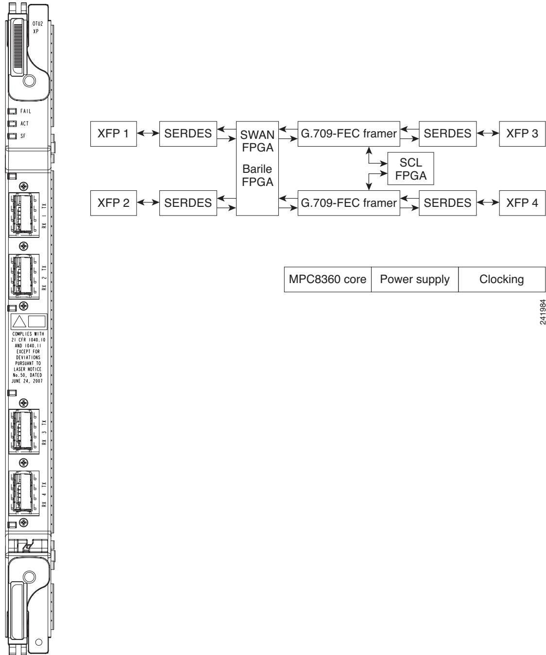
Figure 10-34 OTU2_XP Card Faceplate and Block Diagram
