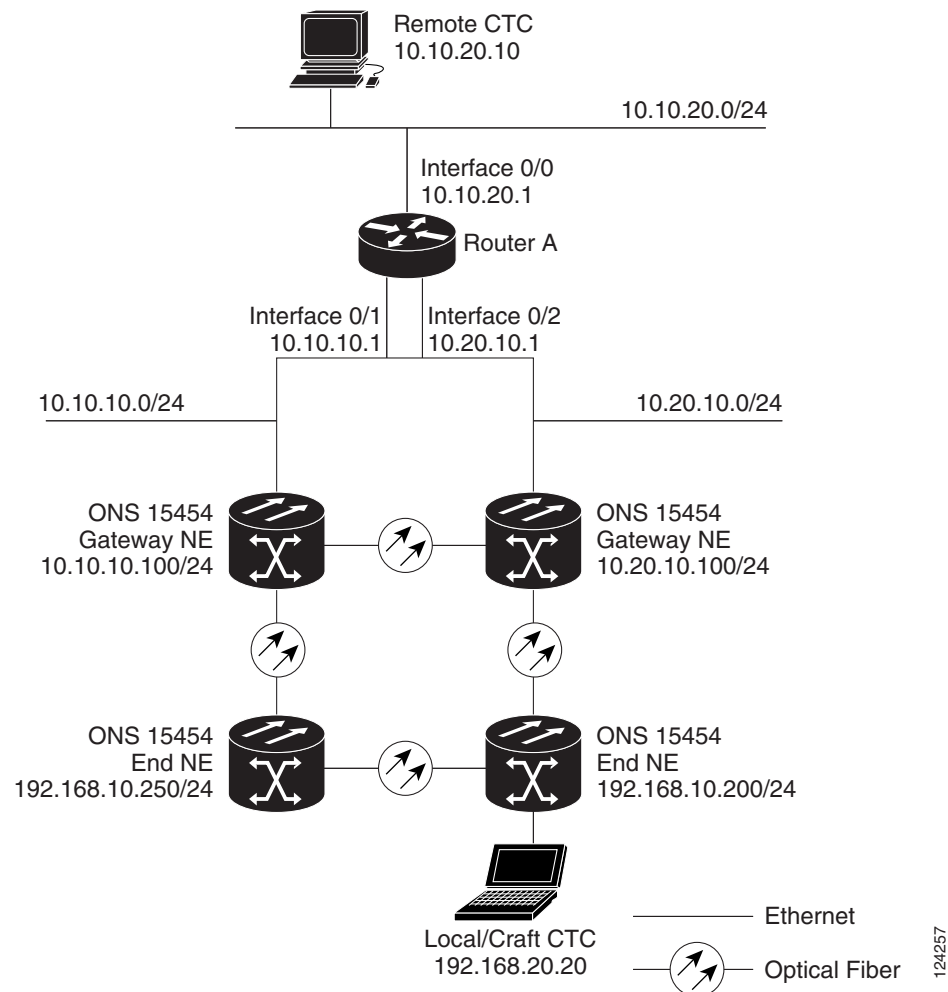
Figure 17-14 Scenario 8: Dual GNEs on Different Subnets (ANSI and ETSI)
