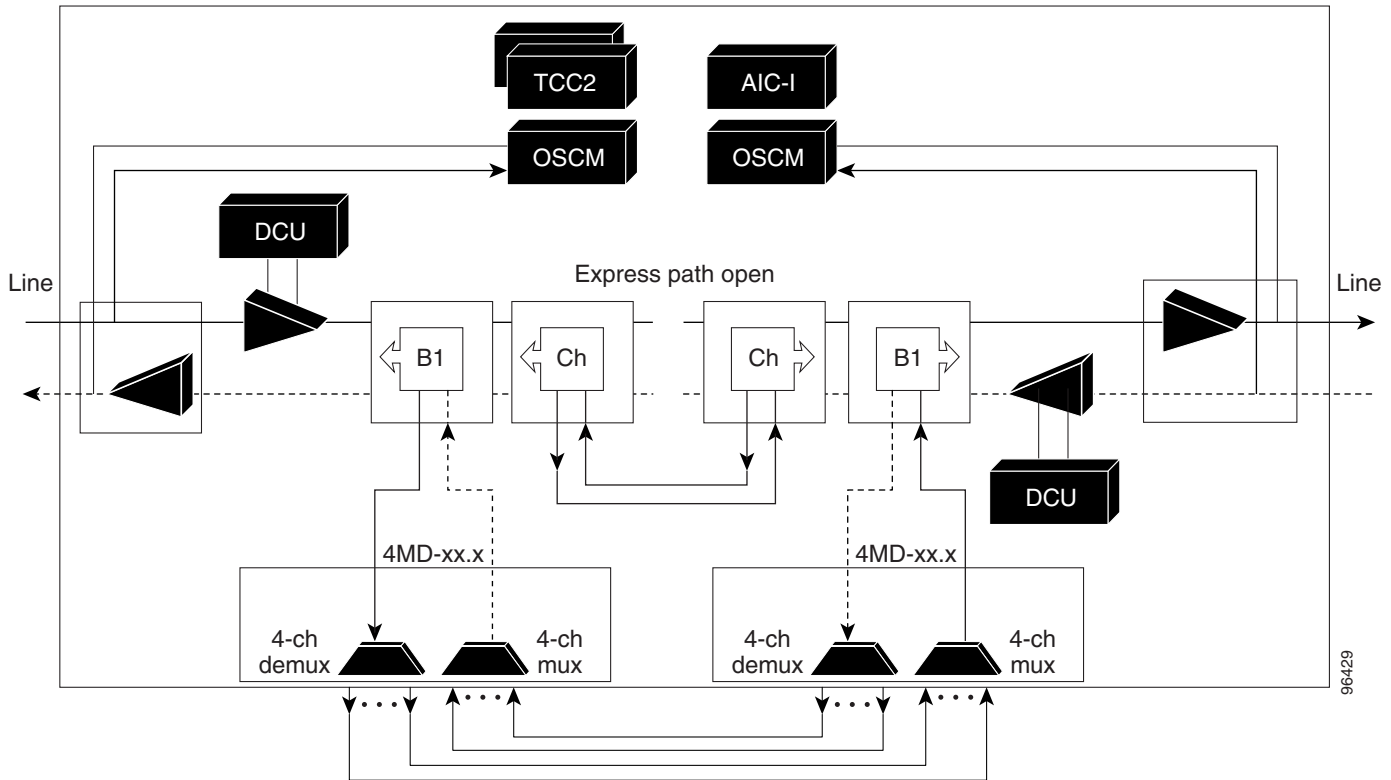
Figure 11-30 Anti-ASE Node Channel Flow Example
