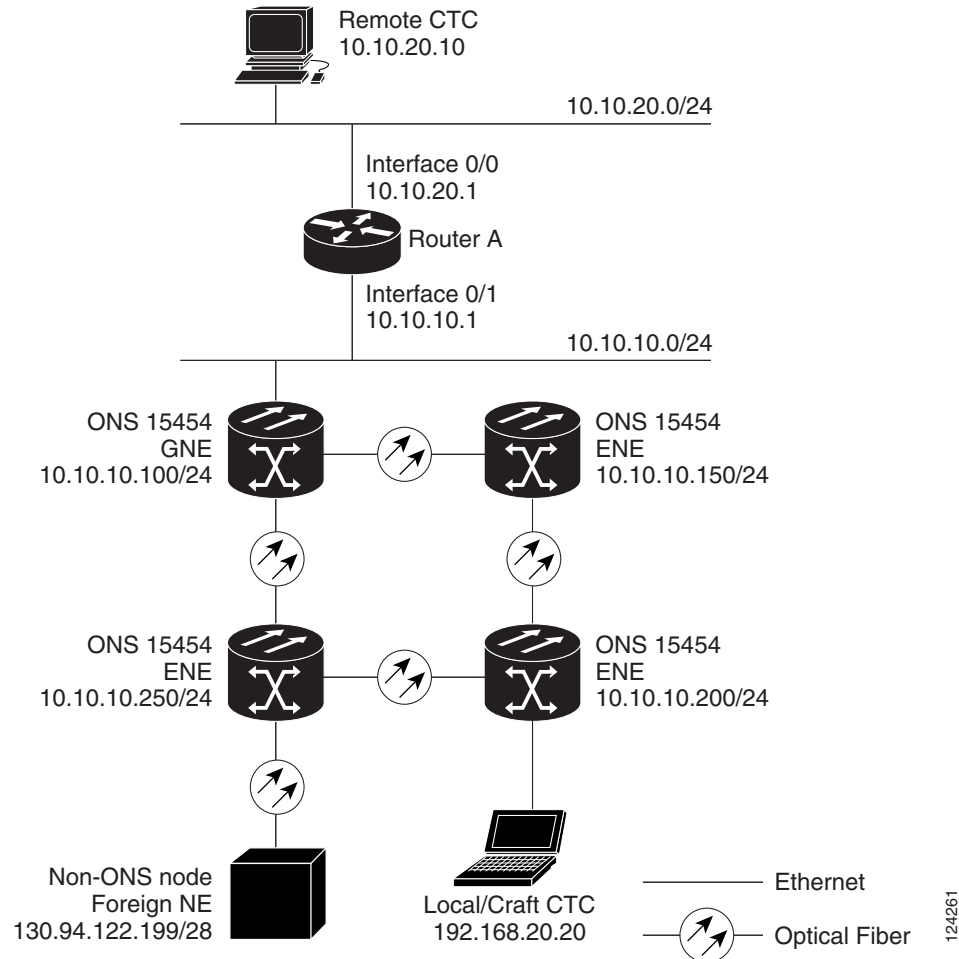
Figure 17-25 Proxy and Firewall Tunnels for Foreign Terminations
