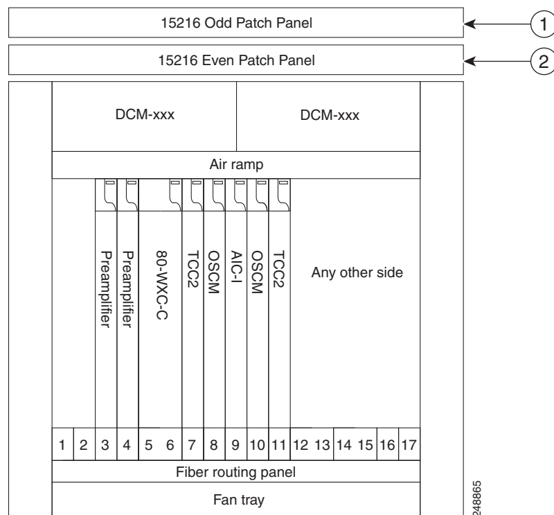
Figure 11-17 80-Channel n-degree ROADM node with Omni-directional Side
