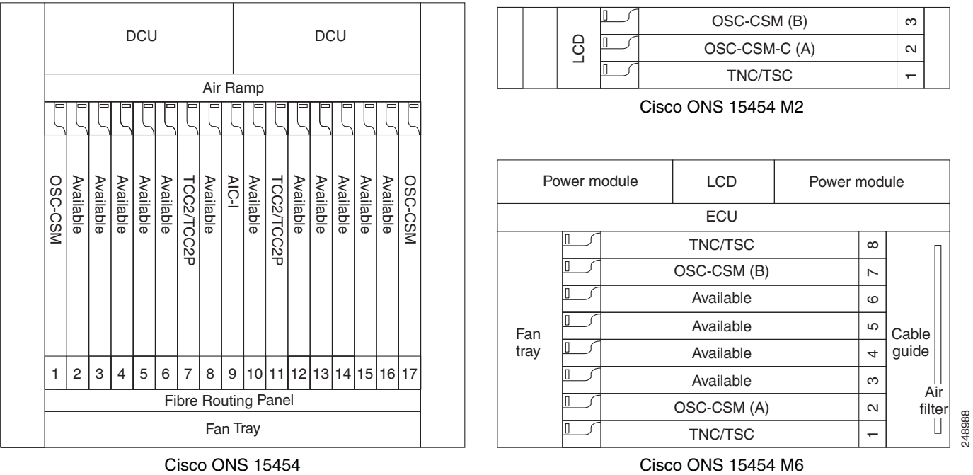
Figure 11-36 OSC Regeneration Line Node Configuration Example - Cisco ONS 15454, Cisco ONS 15454 M6, and Cisco ONS 15454 M2
