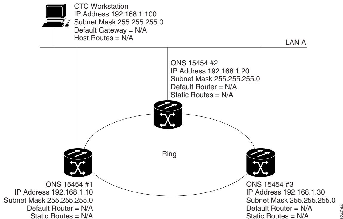
Figure 17-1 Scenario 1: CTC and ONS 15454s on Same Subnet (ANSI and ETSI)
