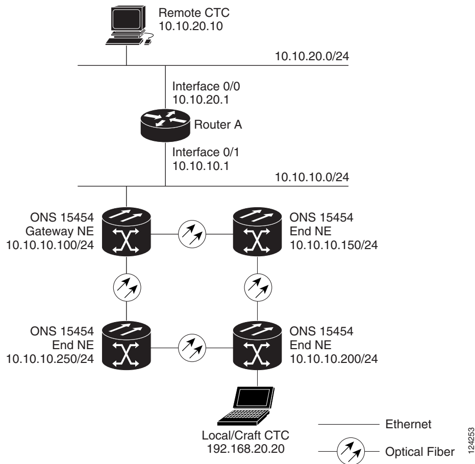
Figure 17-10 Scenario 7: ONS 15454 Proxy Server with GNE and ENEs on the Same Subnet (ANSI and ETSI)
