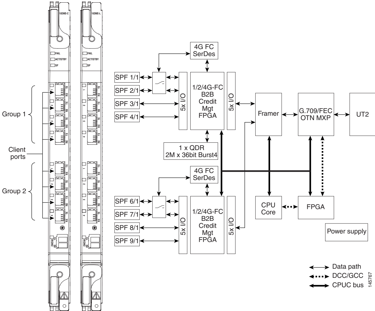
Figure 10-26 MXP_MR_10DME_C and MXP_MR_10DME_L Faceplates and Block Diagram
