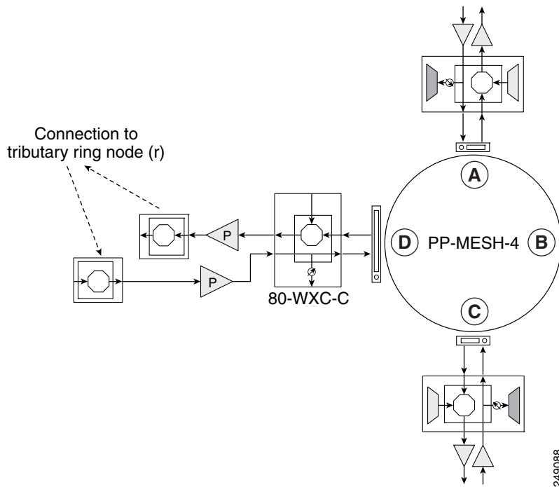
Figure 12-11 Colorless and Omni-directional n-Degree ROADM Node
