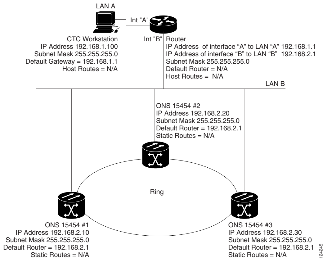
Figure 17-2 Scenario 2: CTC and ONS 15454s Connected to Router (ANSI and ETSI)
