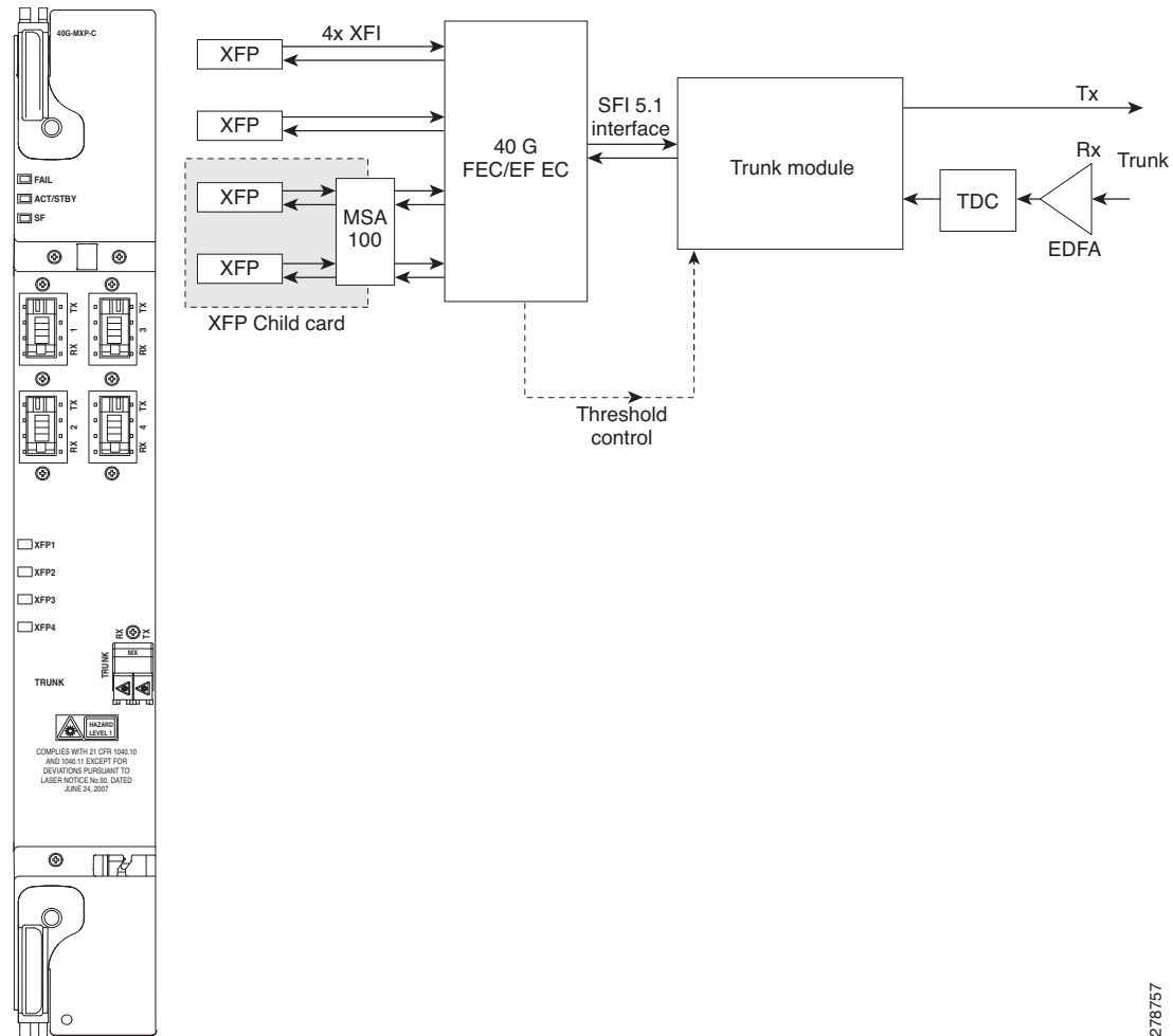
Figure 10-28 Faceplate and Block Diagram of the 40G-MXP-C, 40E-MXP-C, and 40ME-MXP-C Cards
