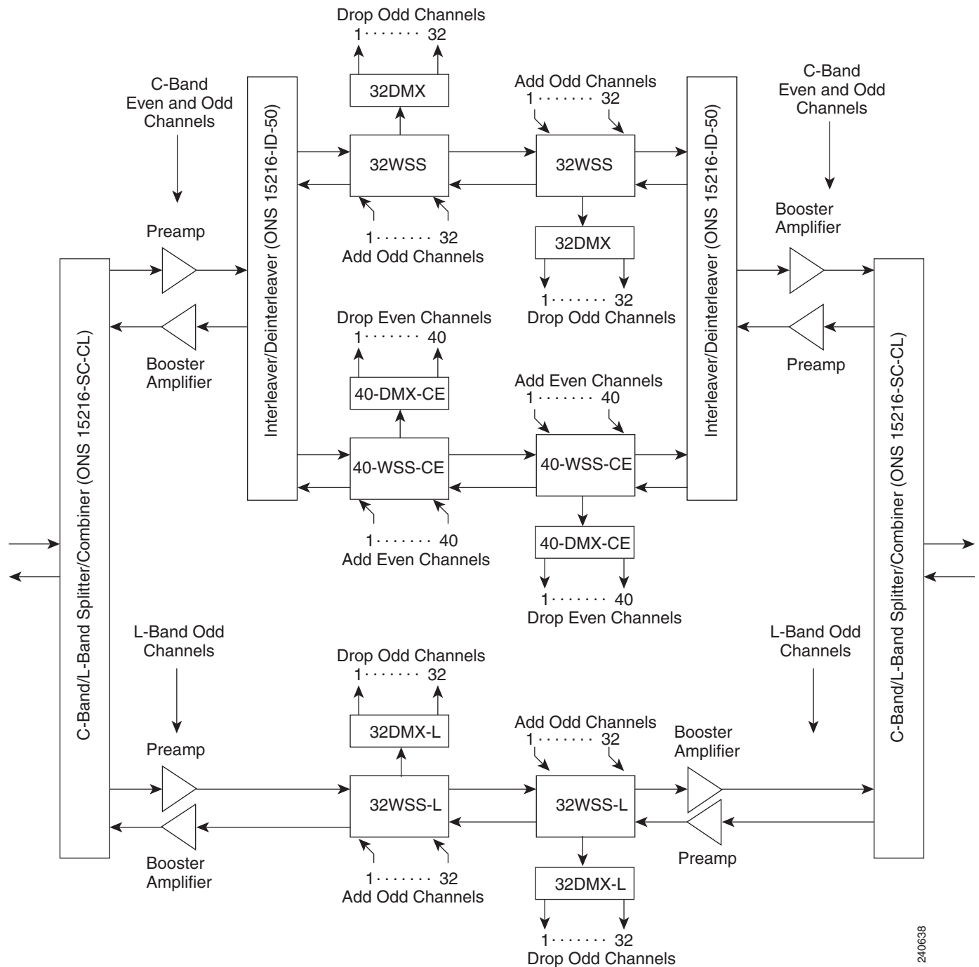
Figure 12-44 104-Channel C-Band plus L-Band ROADM Node
