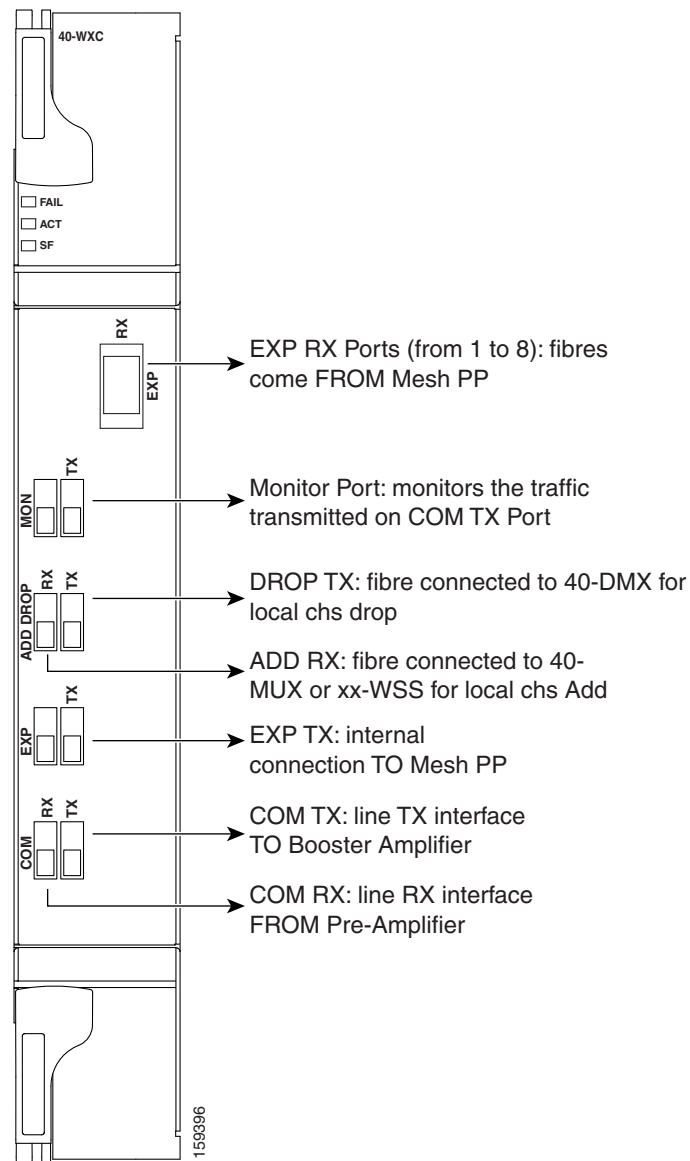
Figure 9-34 40-WXC-C Faceplate
