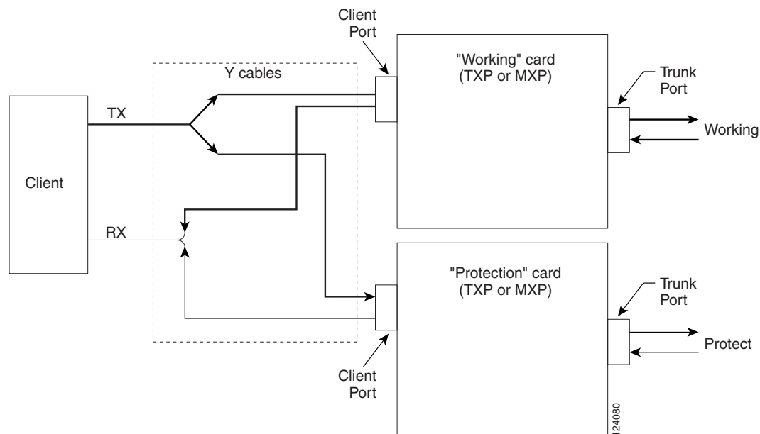
Figure 10-38 Y-Cable Protection
