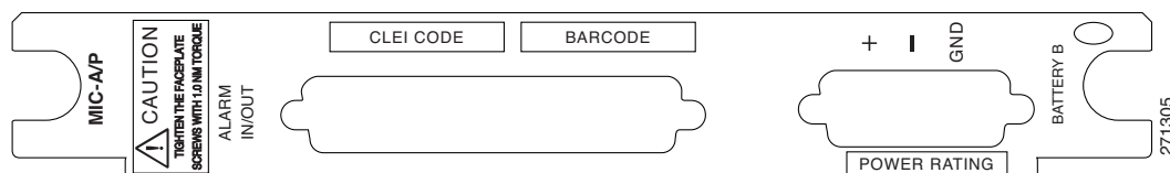
Figure 2-10 MIC-A/P Faceplate
