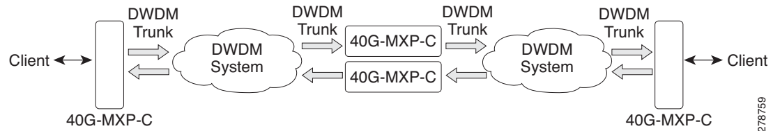
Figure 10-27 40G-MXP-C, 40E-MXP-C, and 40ME-MXP-C Cards in Unidirectional Regeneration Configuration
