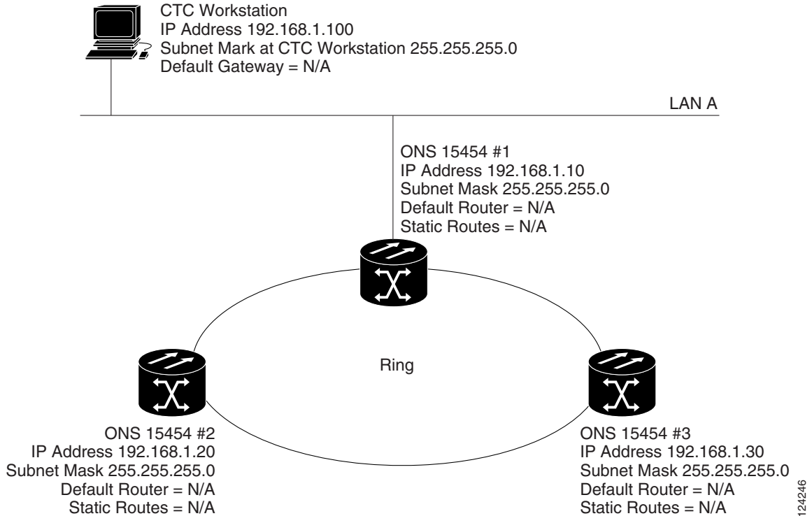
Figure 17-3 Scenario 3: Using Proxy ARP (ANSI and ETSI)
