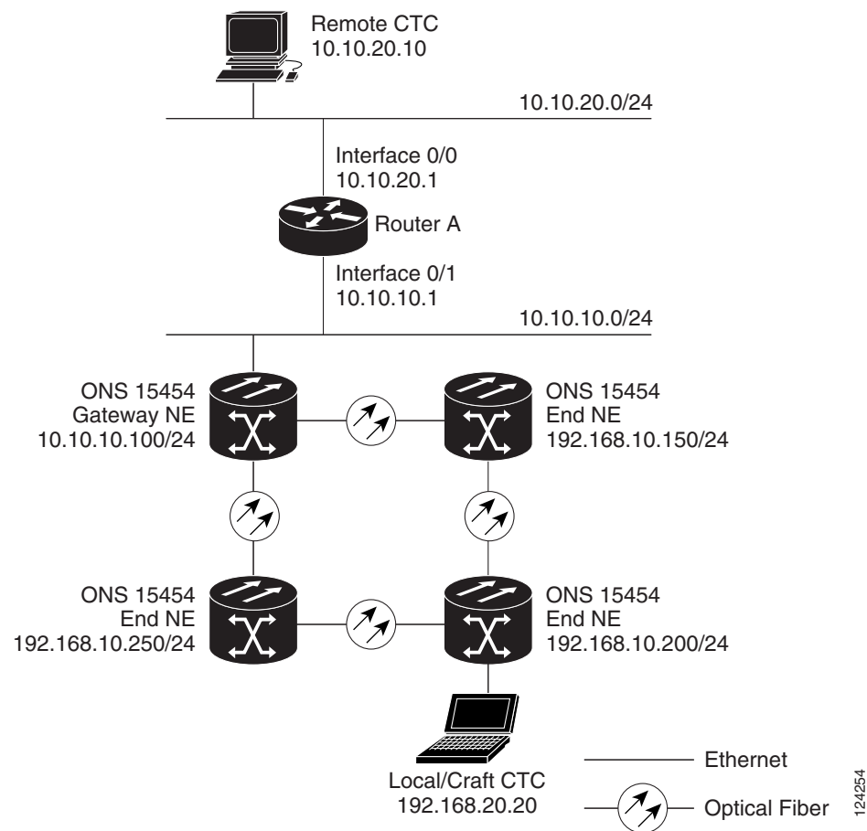
Figure 17-11 Scenario 7: ONS 15454 Proxy Server with GNE and ENEs on Different Subnets (ANSI and ETSI)
