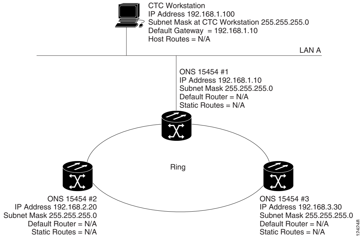
Figure 17-5 Scenario 4: Default Gateway on a CTC Computer (ANSI and ETSI)
