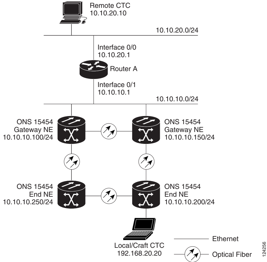
Figure 17-13 Scenario 8: Dual GNEs on the Same Subnet (ANSI and ETSI)
