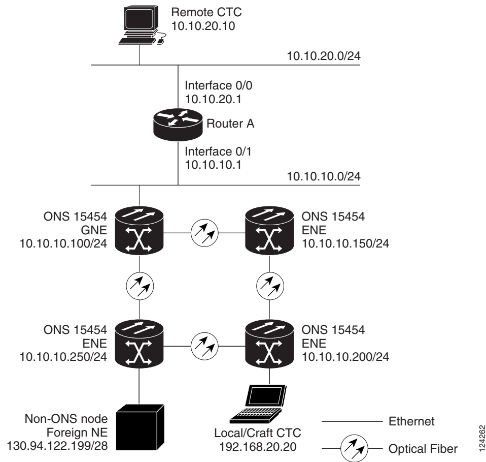
Figure 17-26 Foreign Node Connection to an ENE Ethernet Port
