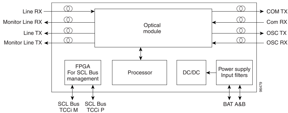
Figure 4-14 OPT-BST-E Block Diagram
