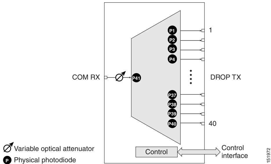
Figure 9-21 40-DMX-C Optical Module Functional Block Diagram
