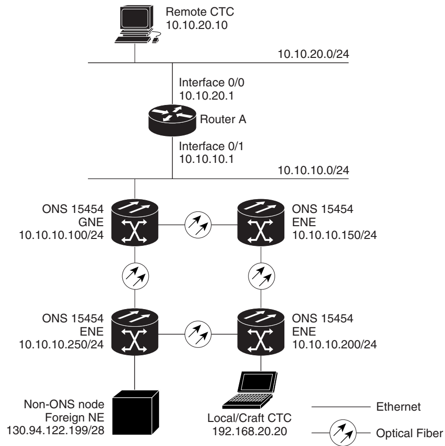
Figure 17-26 Foreign Node Connection to an ENE Ethernet Port
