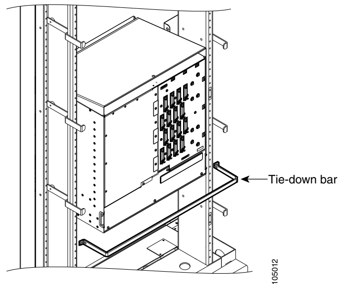
Figure 1-52 Tie-Down Bar on the Cisco ONS 15454 ANSI Shelf Assembly
