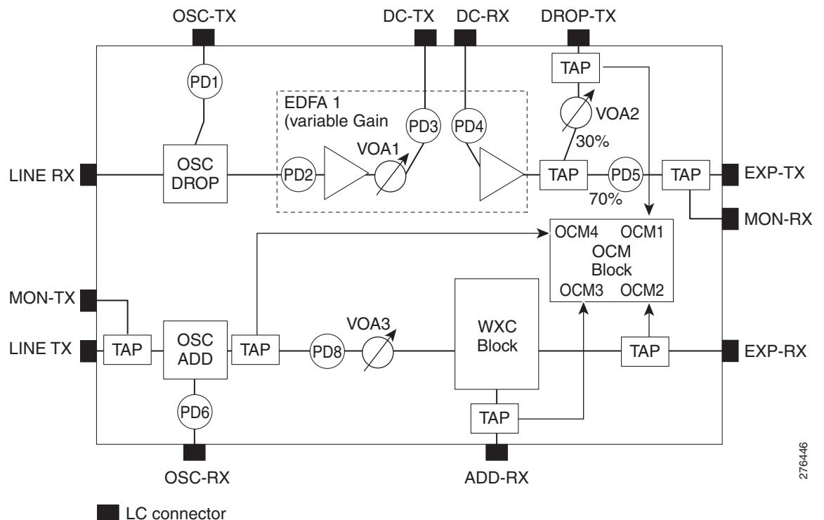
Figure 9-37 40-SMR1-C Block Diagram
