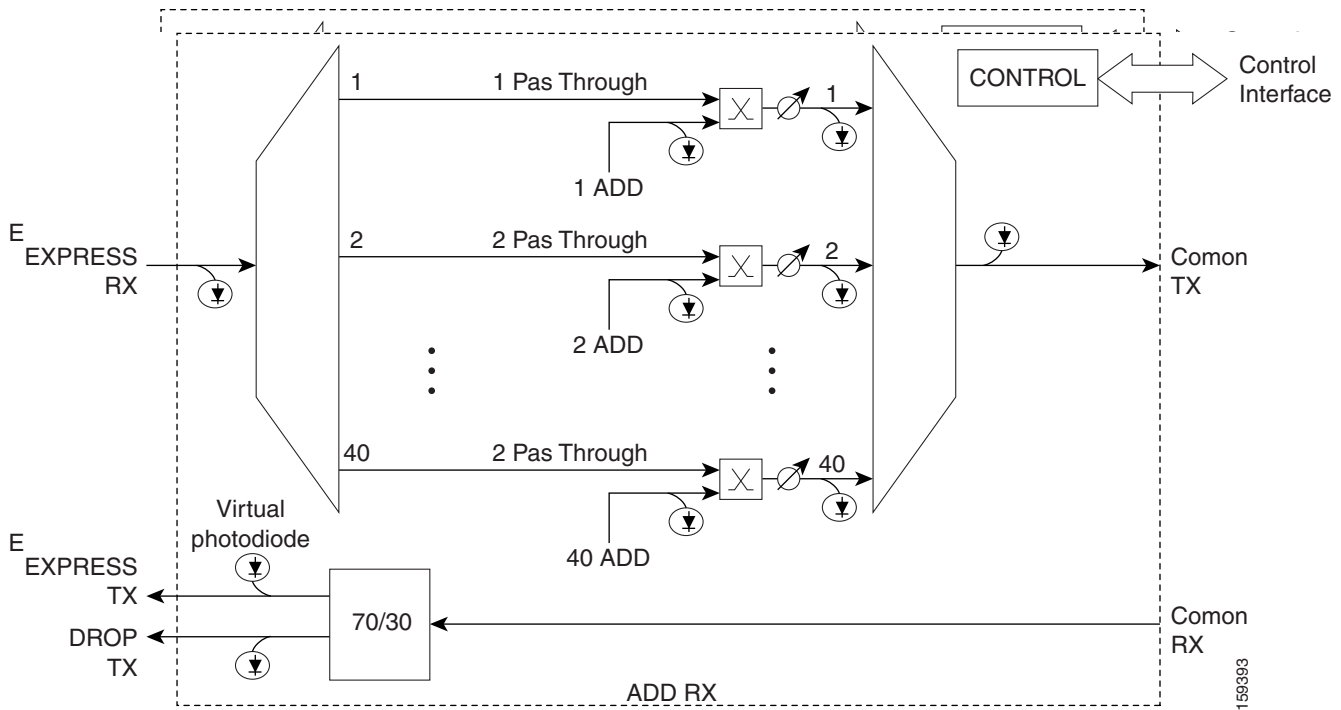
Figure 9-29 40-WSS-C Block Diagram
