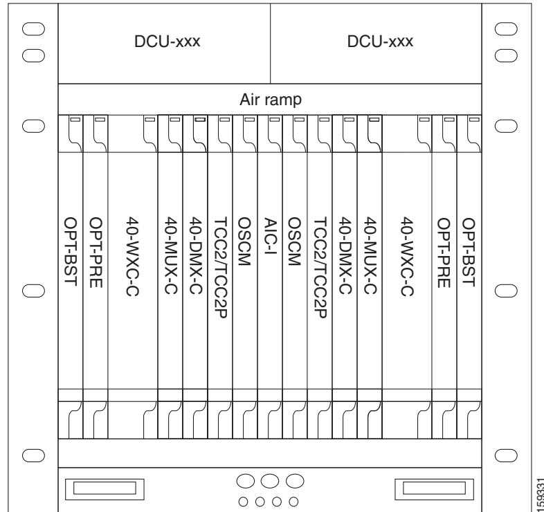
Figure 11-35 Line Termination Mesh Node Shelf
