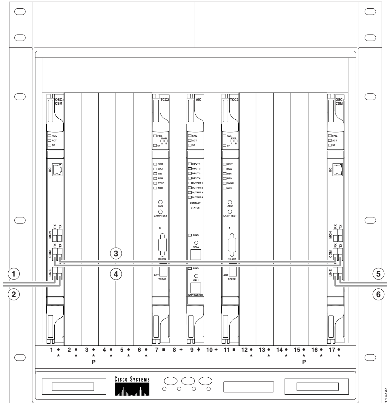
Figure 11-50 Fiberling an OSC Regeneration Node
