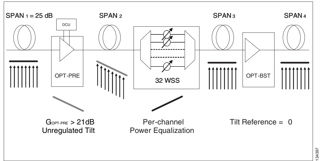
Figure 12-23 System Tilt Compensation With an ROADM Node
