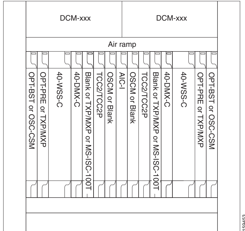
Figure 12-9 Multiring Network
