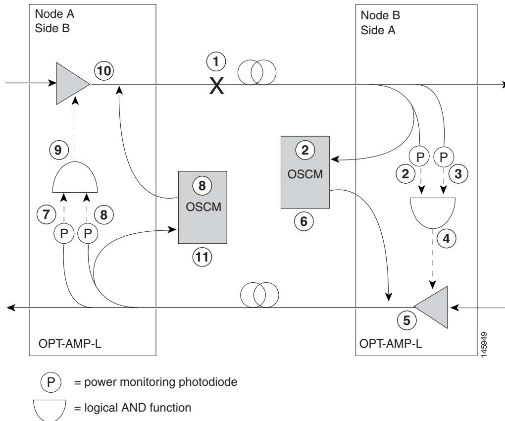
Figure 12-15 Nodes Using OPT-AMP Cards
