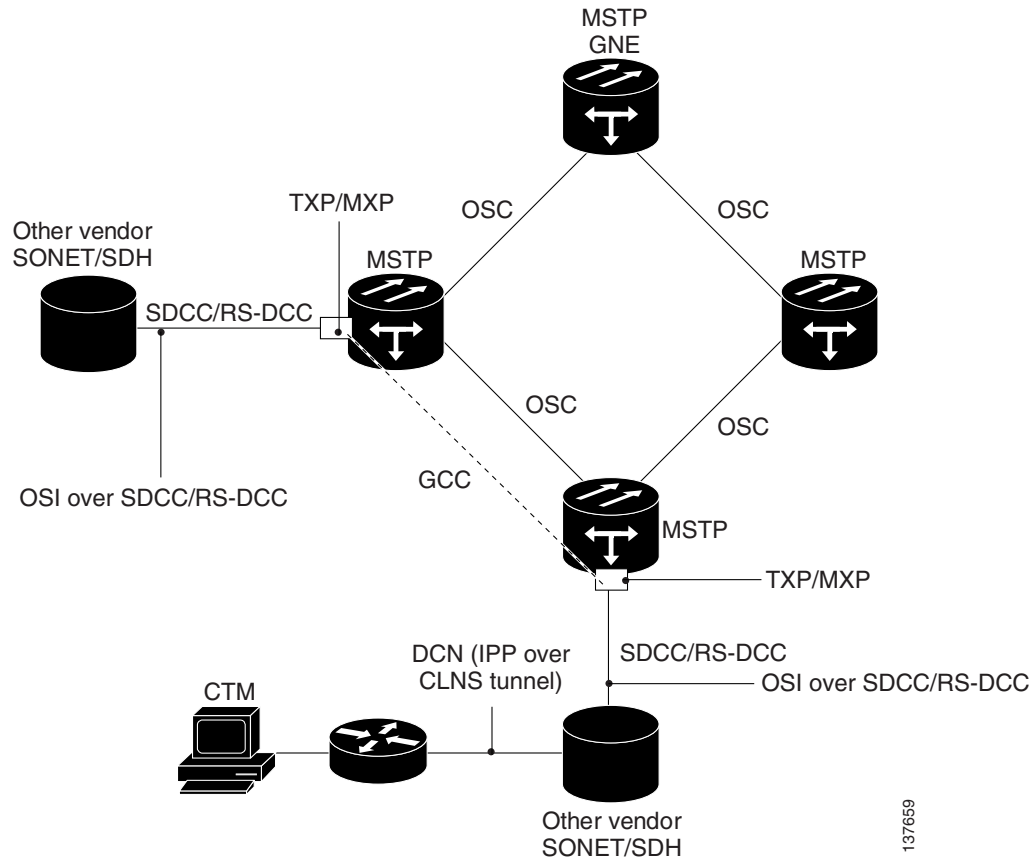
Figure 17-30 OSI/IP Scenario 4
