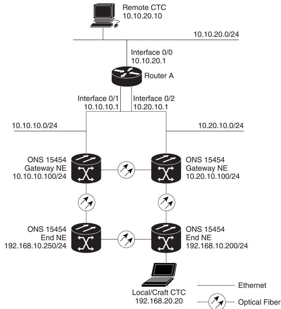
Figure 17-14 Scenario 8: Dual GNEs on Different Subnets (ANSI and ETSI)
