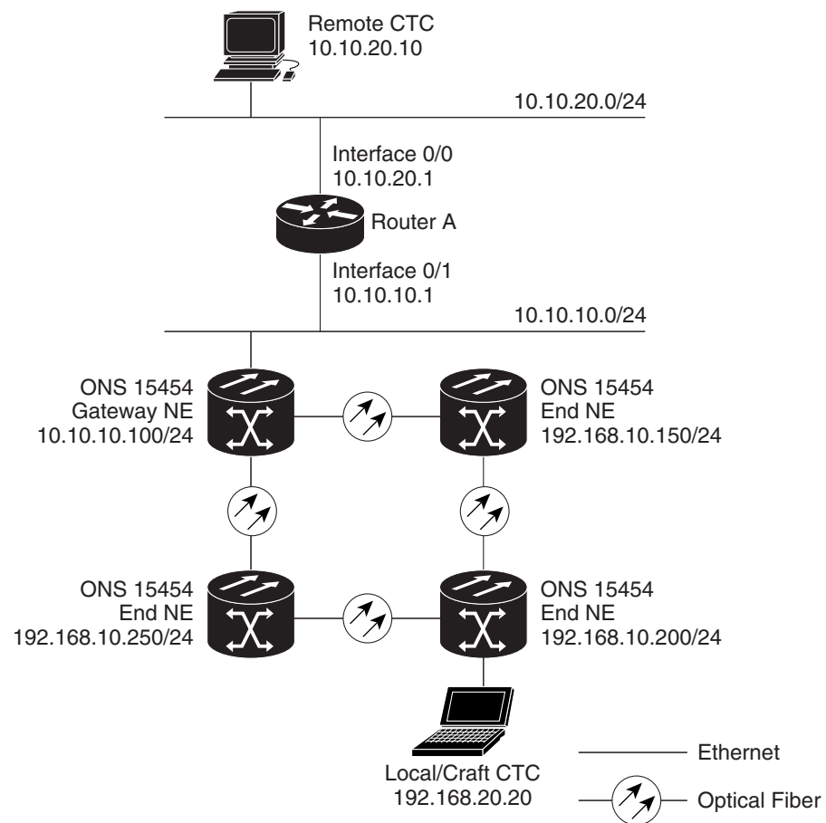
Figure 17-11 Scenario 7: ONS 15454 Proxy Server with GNE and ENEs on Different Subnets (ANSI and ETSI)
