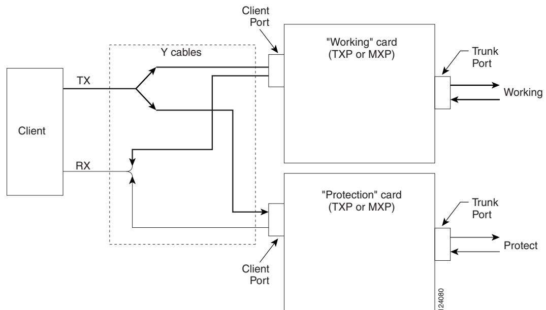
Figure 9-32 Y-Cable Protection
