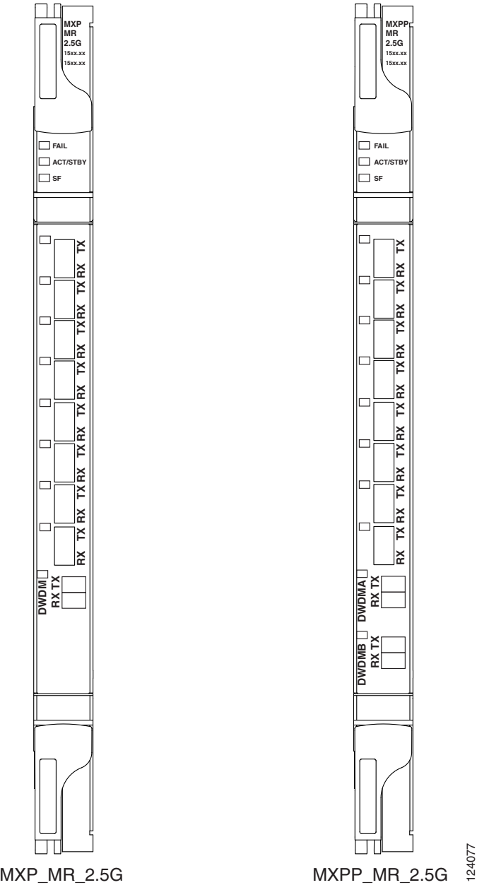
Figure 9-23 MXP_MR_2.5G and MXPP_MR_2.5G Faceplates
