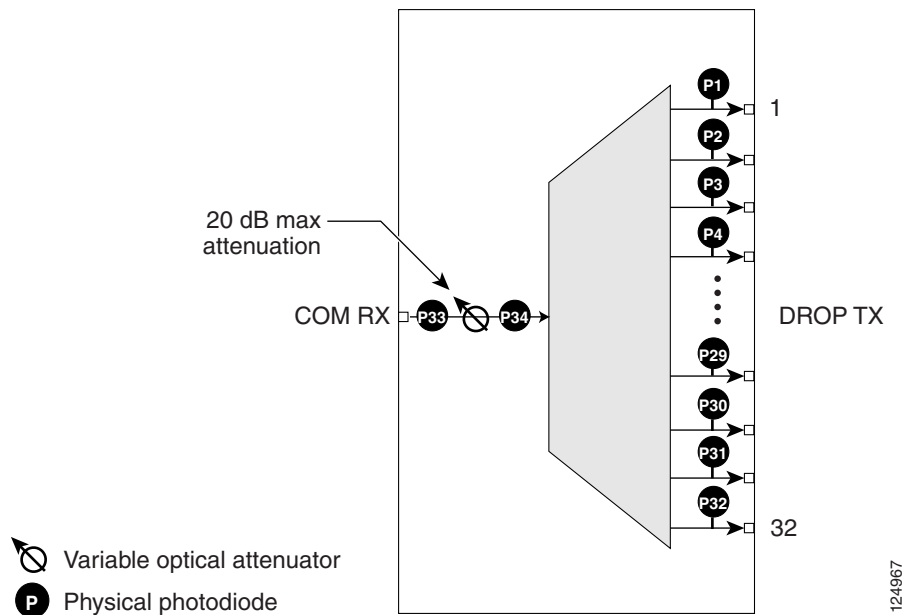
Figure 8-18 32DMX-L Optical Module Functional Block Diagram
