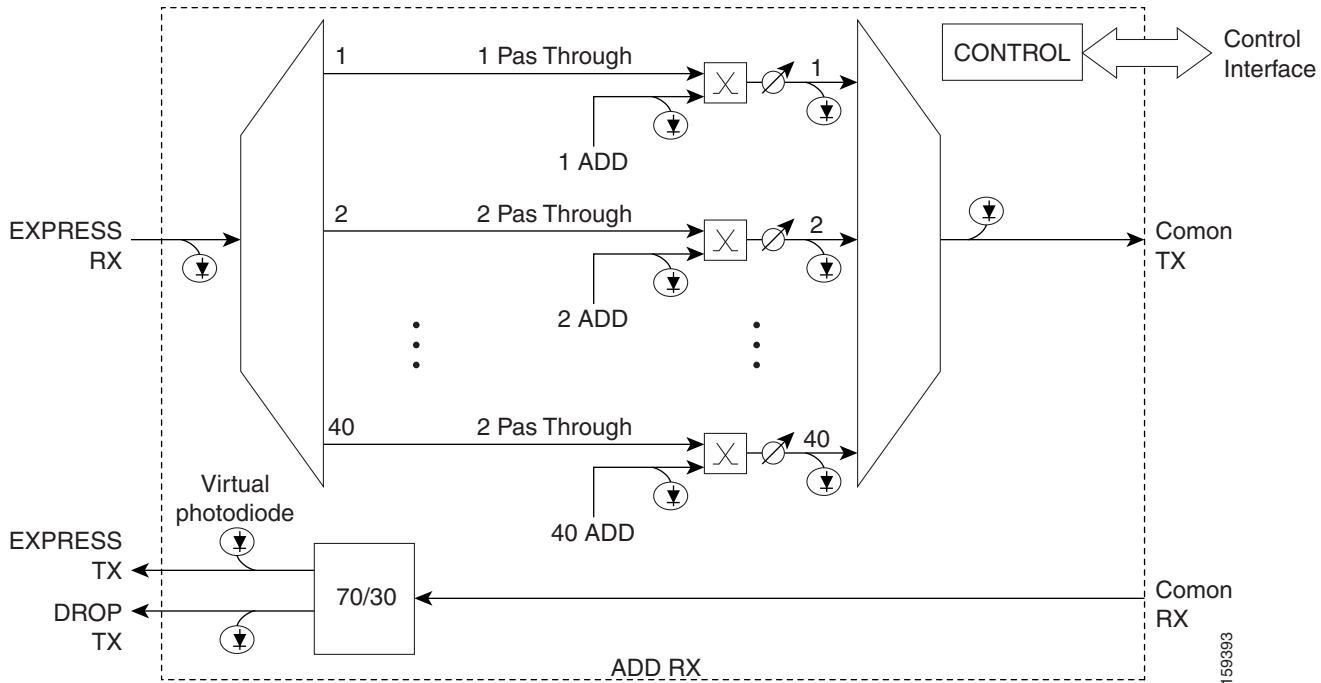
Figure 8-29 40-WSS-C Block Diagram
