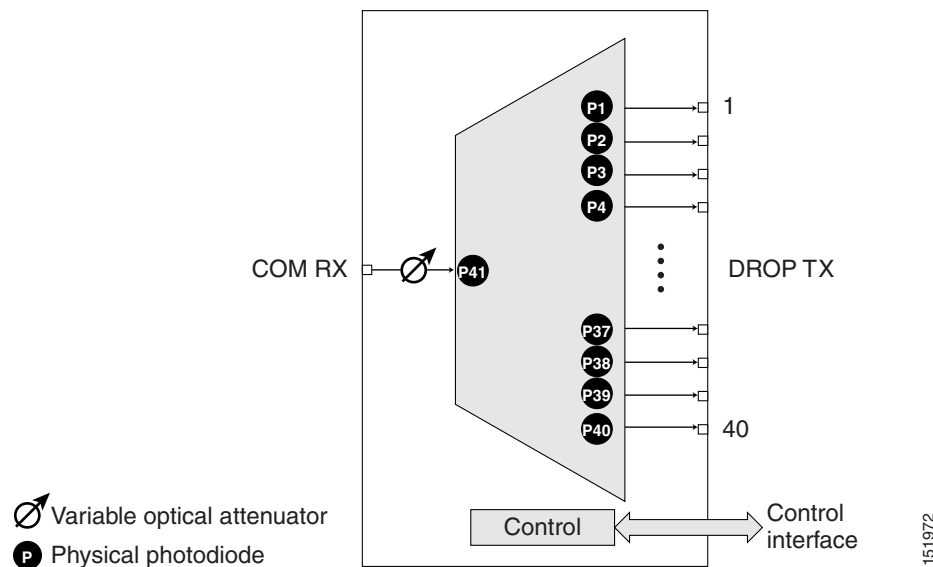
Figure 8-21 40-DMX-C Optical Module Functional Block Diagram
