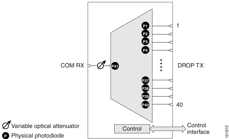
Figure 8-24 40-DMX-CE Card Optical Module Functional Block Diagram
