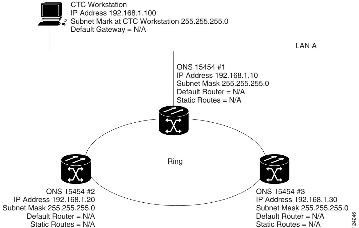
Figure 16-3 Scenario 3: Using Proxy ARP (ANSI and ETSI)
