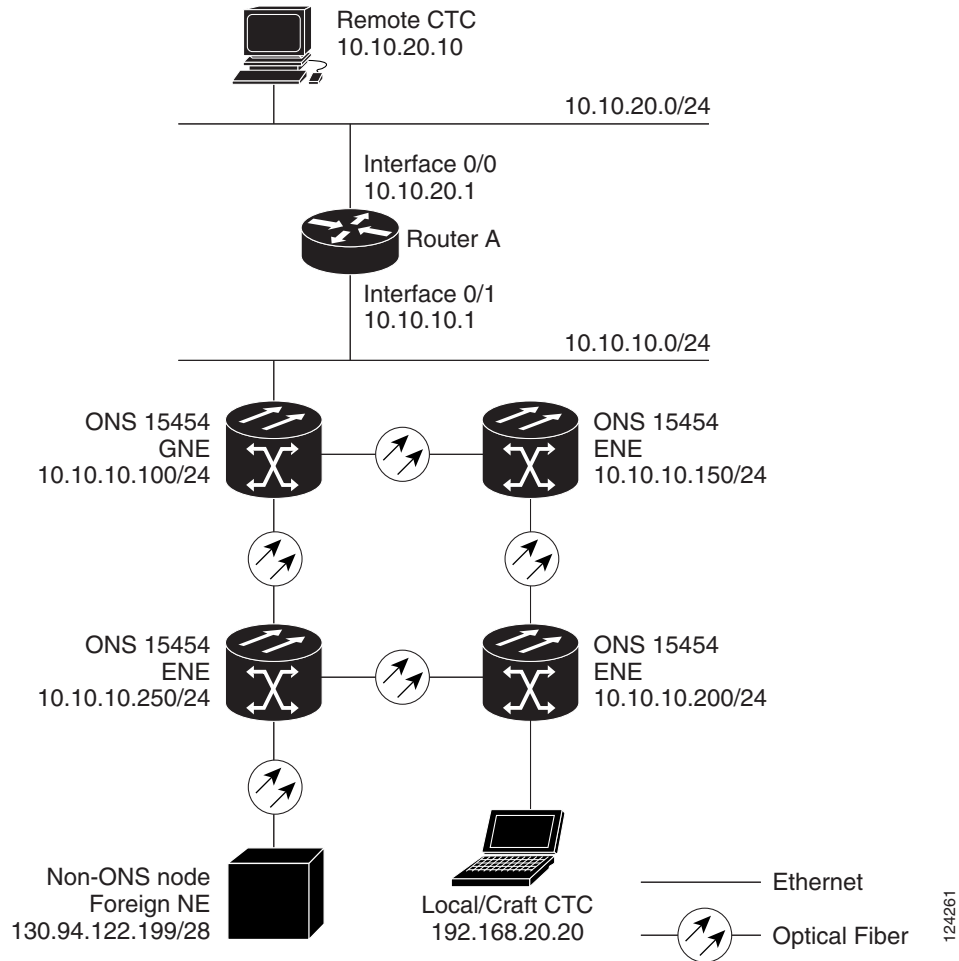
Figure 16-25 Proxy and Firewall Tunnels for Foreign Terminations
