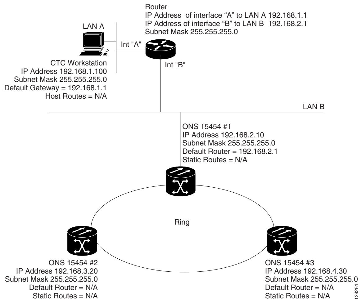
Figure 16-8 Scenario 6: OSPF Enabled (ANSI and ETSI)
