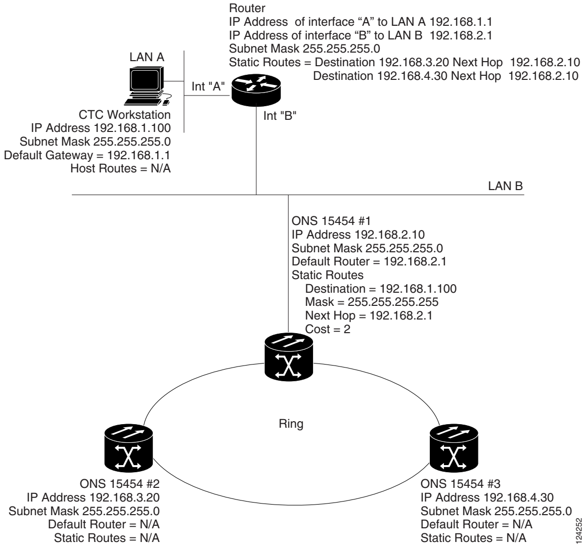
Figure 16-9 Scenario 6: OSPF Not Enabled (ANSI and ETSI)
