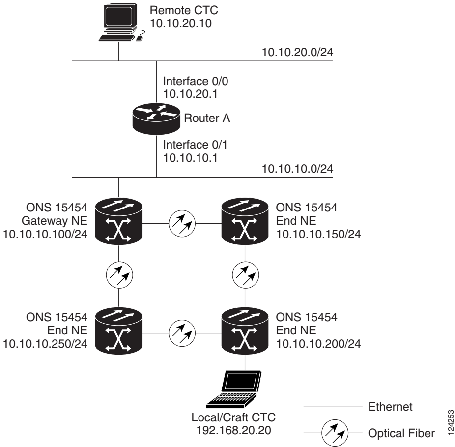
Figure 16-10 Scenario 7: ONS 15454 Proxy Server with GNE and ENEs on the Same Subnet (ANSI and ETSI)
