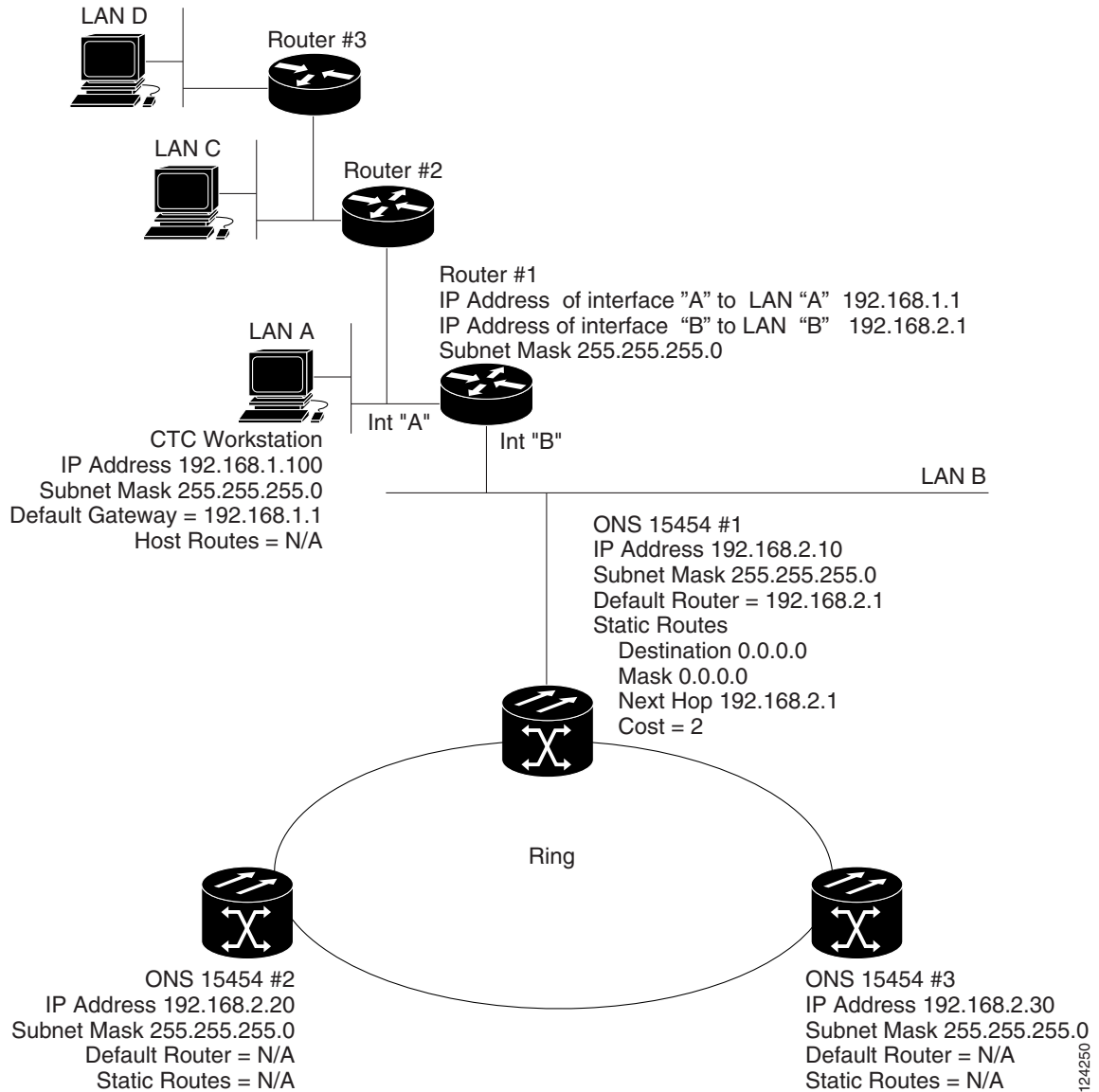
Figure 16-7 Scenario 5: Static Route With Multiple LAN Destinations (ANSI and ETSI)
