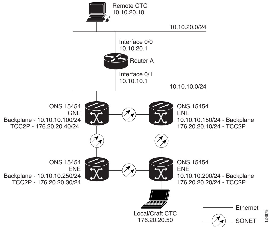
Figure 16-15 Scenario 9: ONS 15454 GNE and ENEs on the Same Subnet with Secure Mode Enabled
