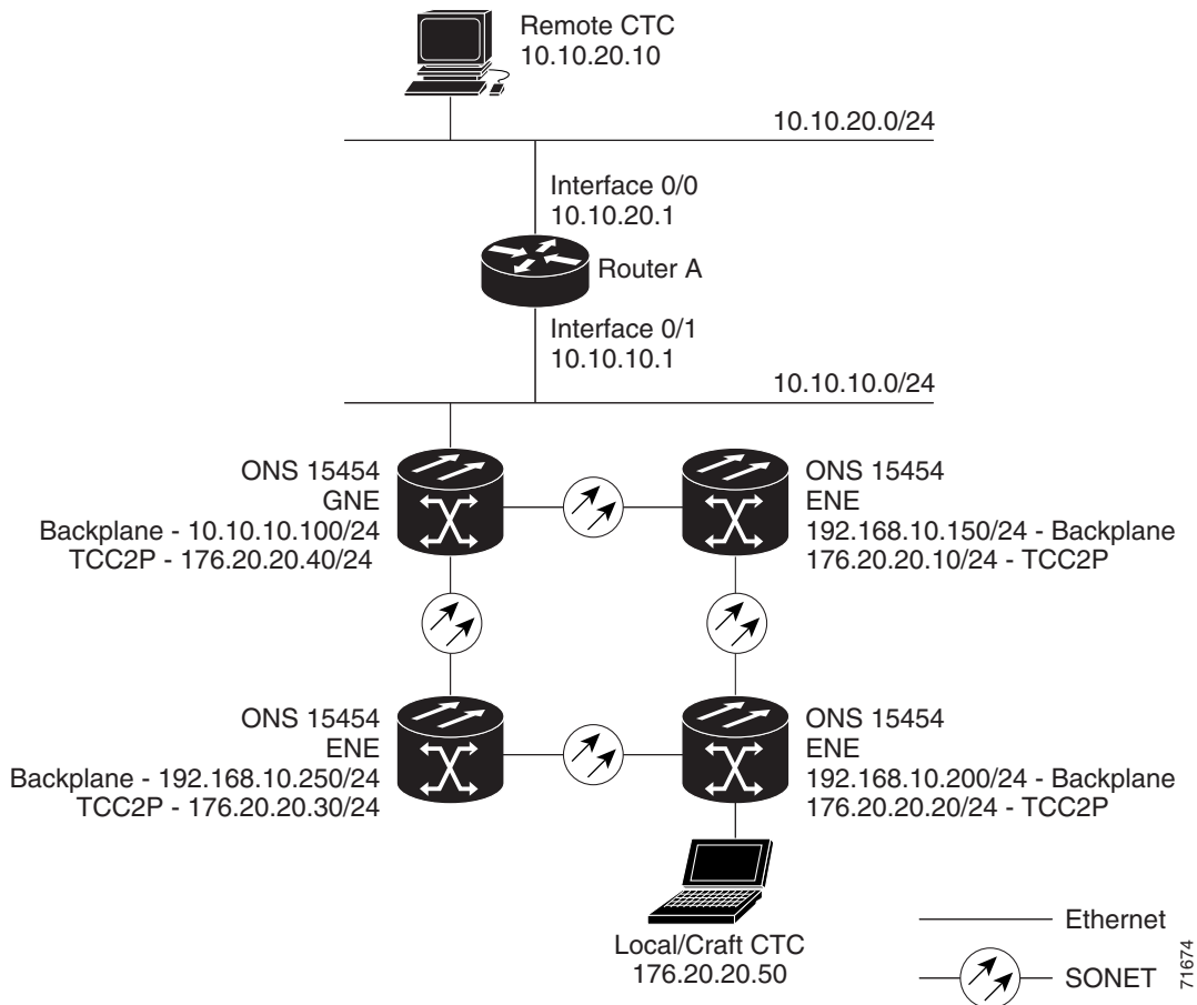
Figure 16-16 Scenario 9: ONS 15454 GNE and ENEs on Different Subnets with Secure Mode Enabled
