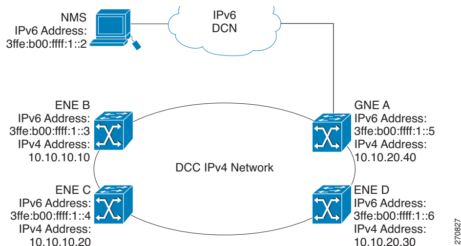
Figure 16-33 IPv6-IPv4 Interaction
