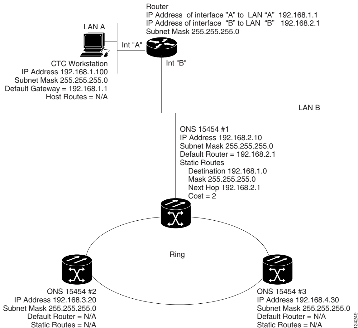
Figure 16-6 Scenario 5: Static Route With One CTC Computer Used as a Destination (ANSI and ETSI)
