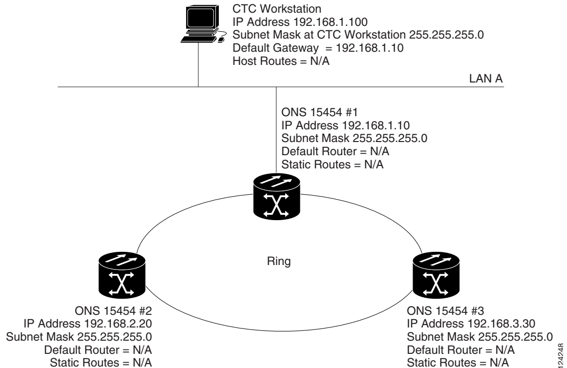
Figure 16-5 Scenario 4: Default Gateway on a CTC Computer (ANSI and ETSI)
