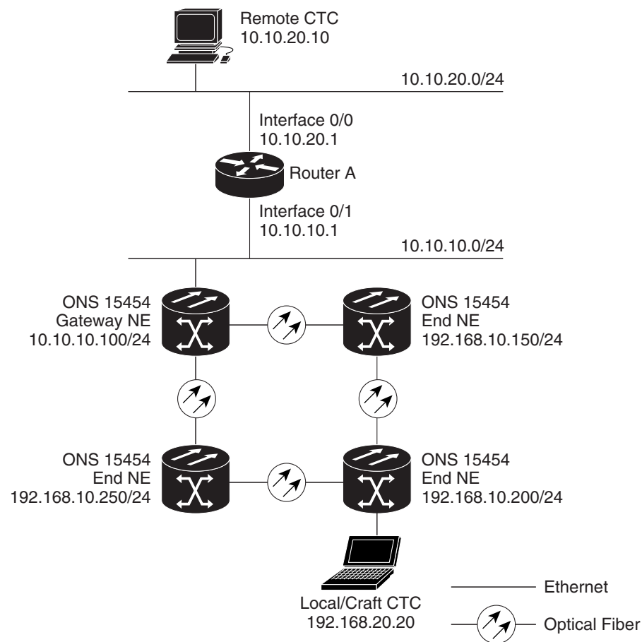
Figure 16-11 Scenario 7: ONS 15454 Proxy Server with GNE and ENEs on Different Subnets (ANSI and ETSI)
