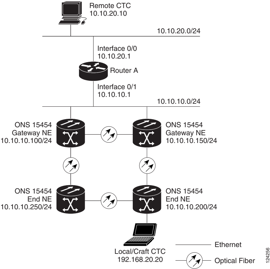
Figure 16-13 Scenario 8: Dual GNEs on the Same Subnet (ANSI and ETSI)
