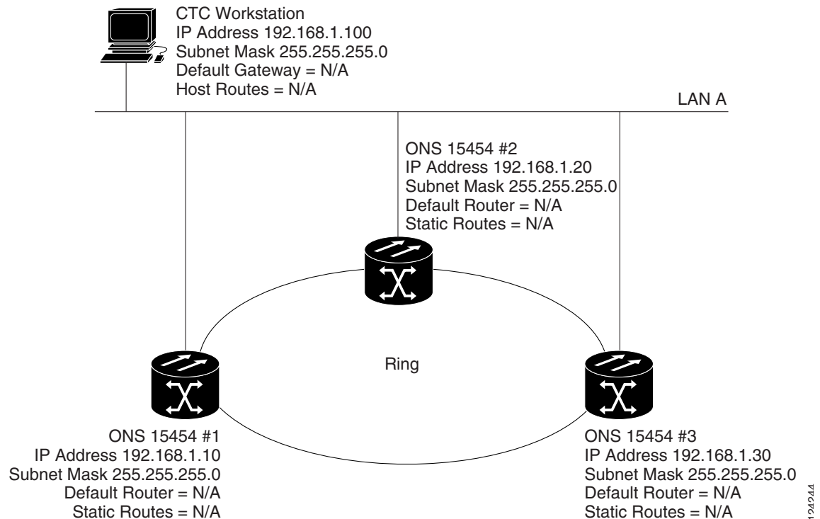
Figure 16-1 Scenario 1: CTC and ONS 15454s on Same Subnet (ANSI and ETSI)
