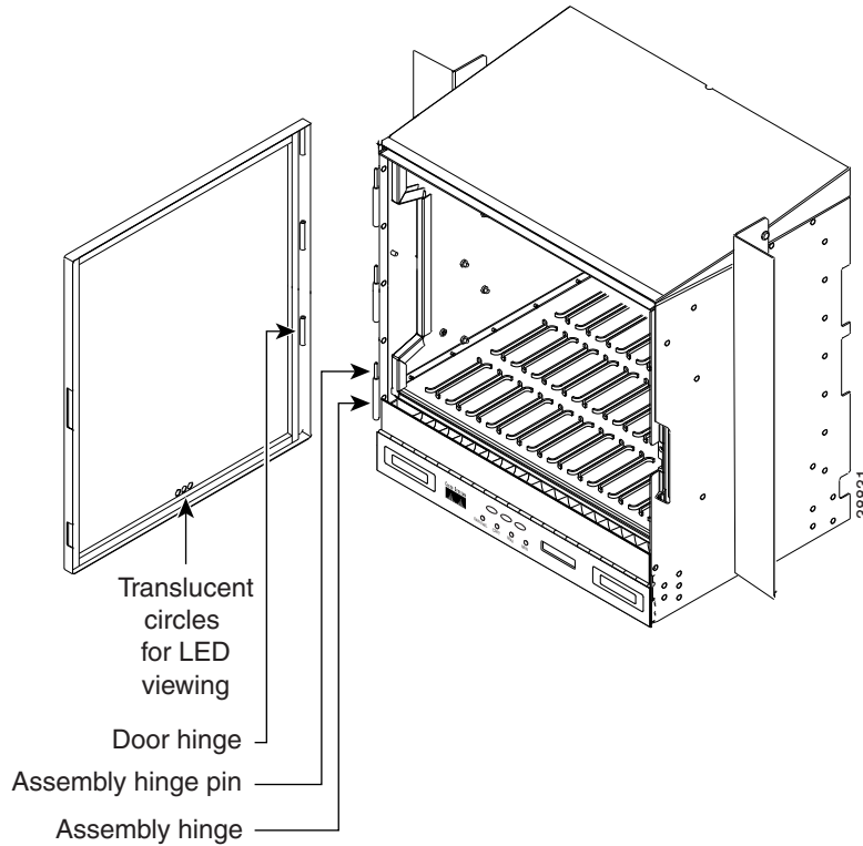
Figure 1-6 Removing the ONS 15454 Front Door
