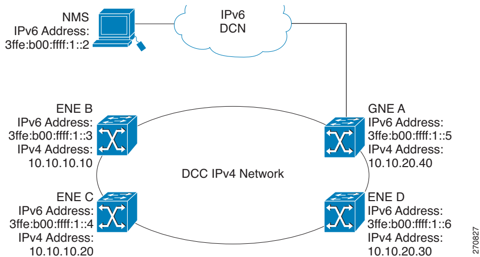
Figure 13-40 IPv6-IPv4 Interaction
