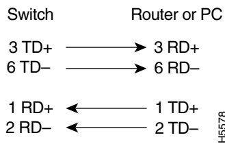
Figure 1-30 Straight-Through Cable
