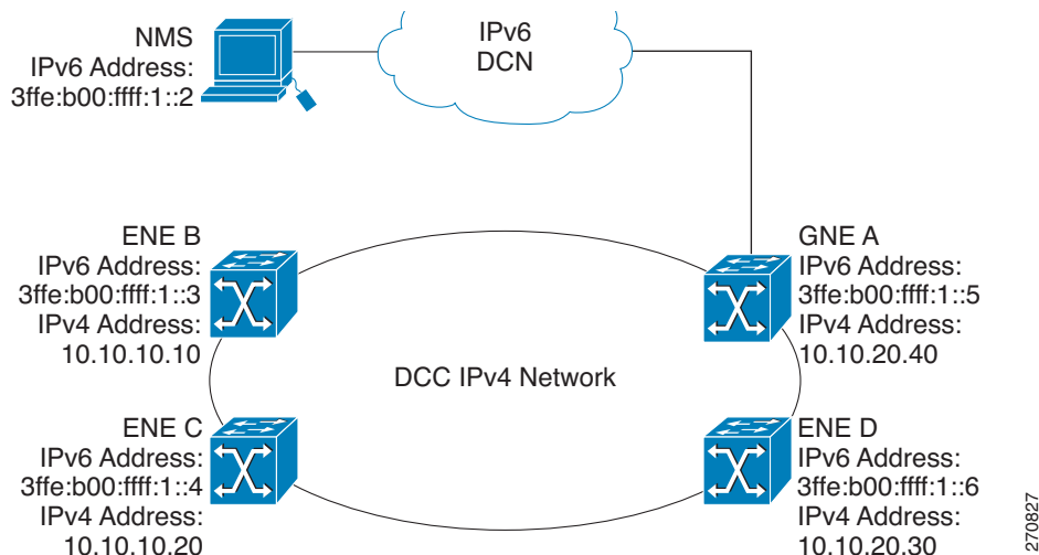
Figure 13-40 IPv6-IPv4 Interaction
