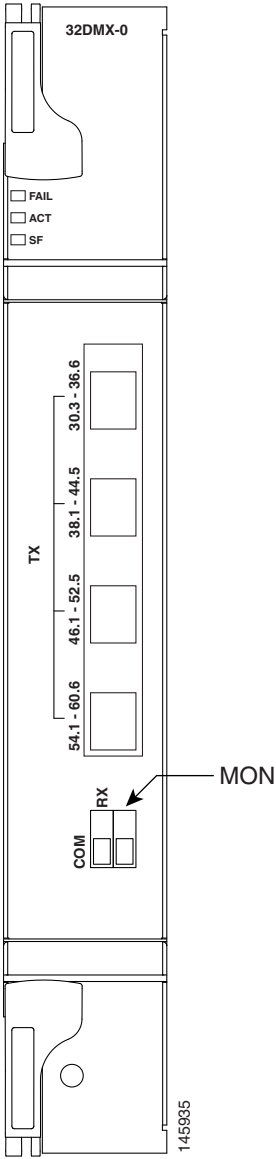
Figure 5-14 32DMX-O Faceplate
