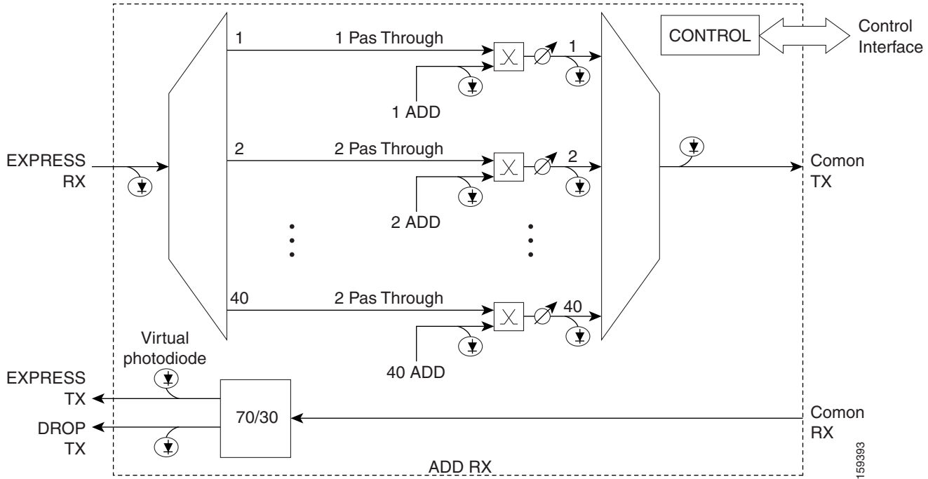
Figure 7-28 40-WSS-C Block Diagram
