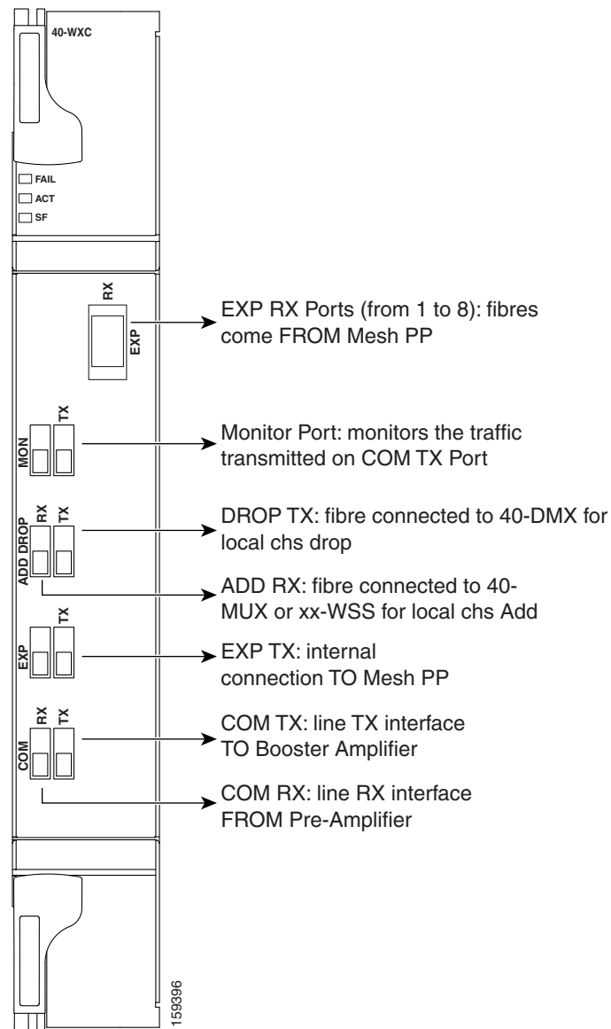
Figure 7-33 40-WXC-C Faceplate
