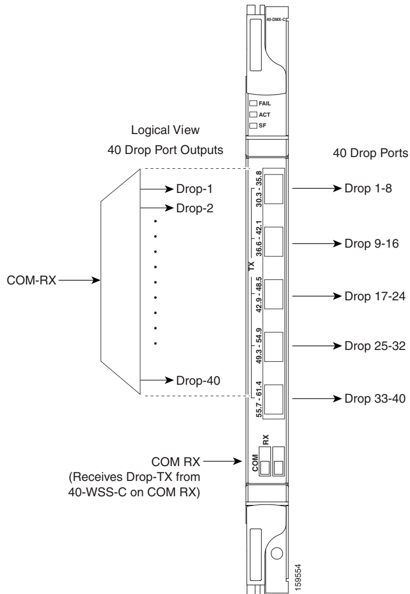
Figure 7-18 40-DMX-C Faceplate
