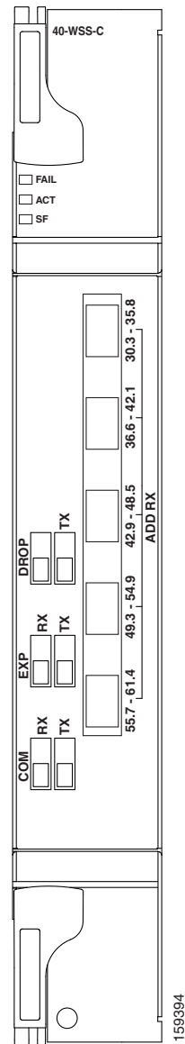
Figure 7-27 40-WSS-C Faceplate
