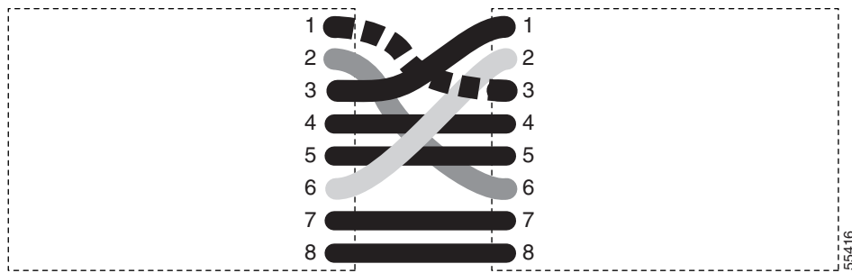
Figure 1-20 Cross-Over Cable Layout
