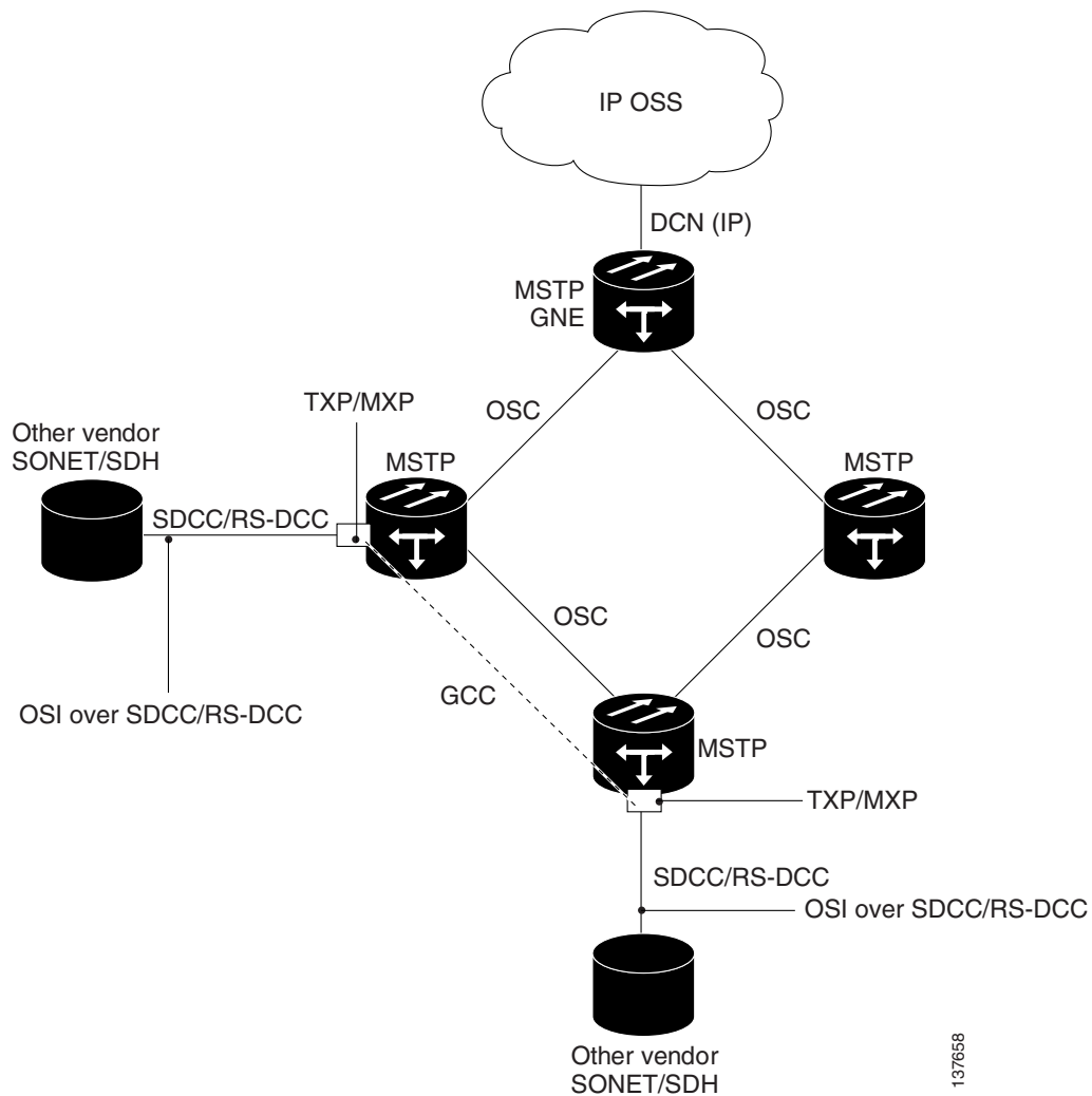
Figure 15-26 OSI/MSTP Scenario 3
