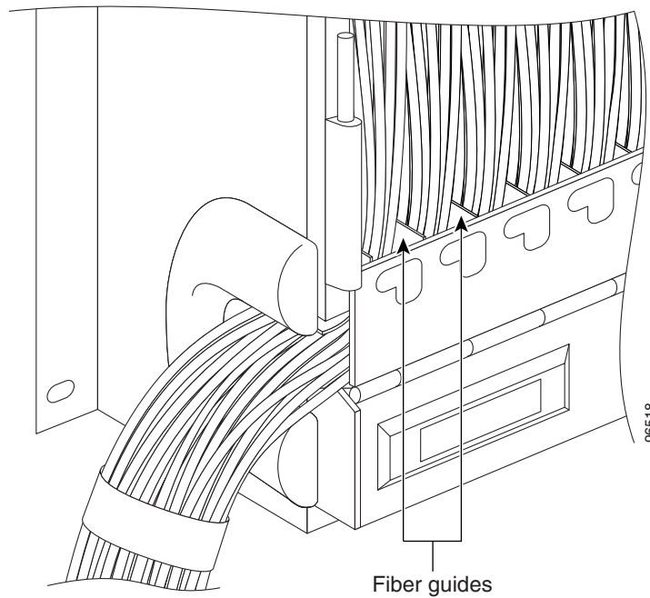
Figure 1-40 Fiber Capacity
