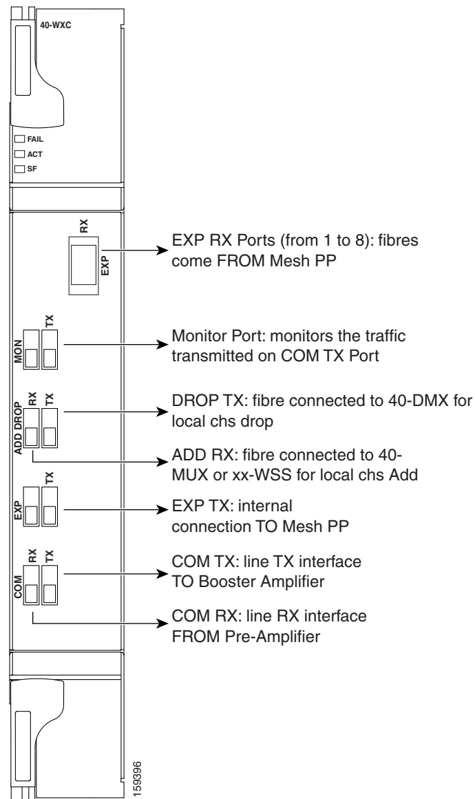
Figure 7-27 40-WXC-C Faceplate
