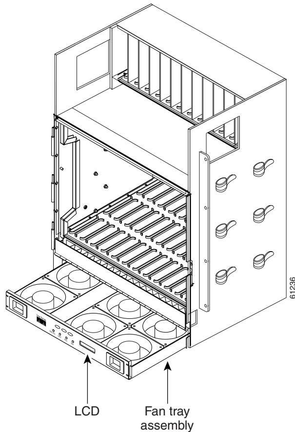
Figure 1-51 Position of the ONS 15454 ETSI Fan-Tray Assembly
