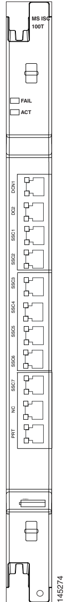
Figure 2-5 MS-ISC-100T Faceplate
