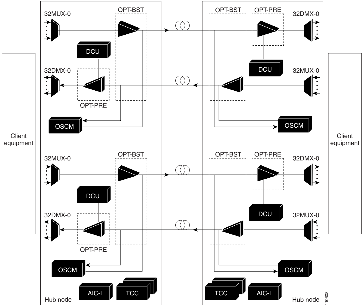
Figure 3-24 1+1 Protected Single-Span Link with Hub Nodes
