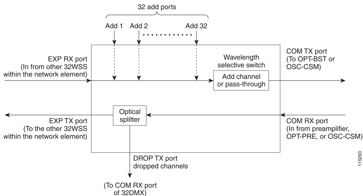
Figure 2-51 32WSS Block Diagram
