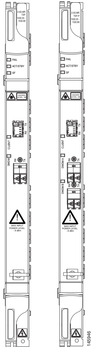
Figure 2-79 TXP_MR_2.5G and TXPP_MR_2.5G Faceplates
