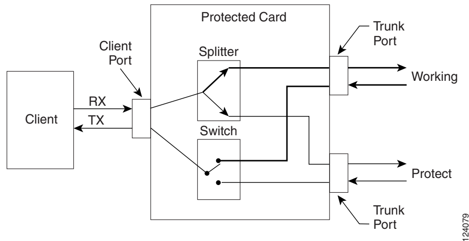
Figure 2-90 Splitter Protection
