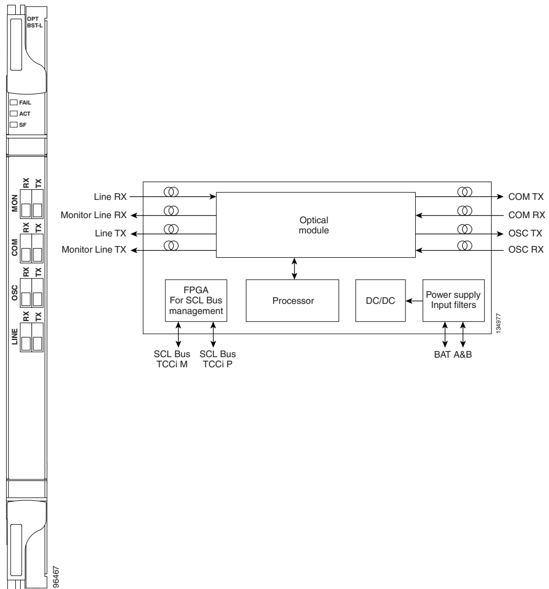
Figure 2-34 OPT-BST-L Faceplate
