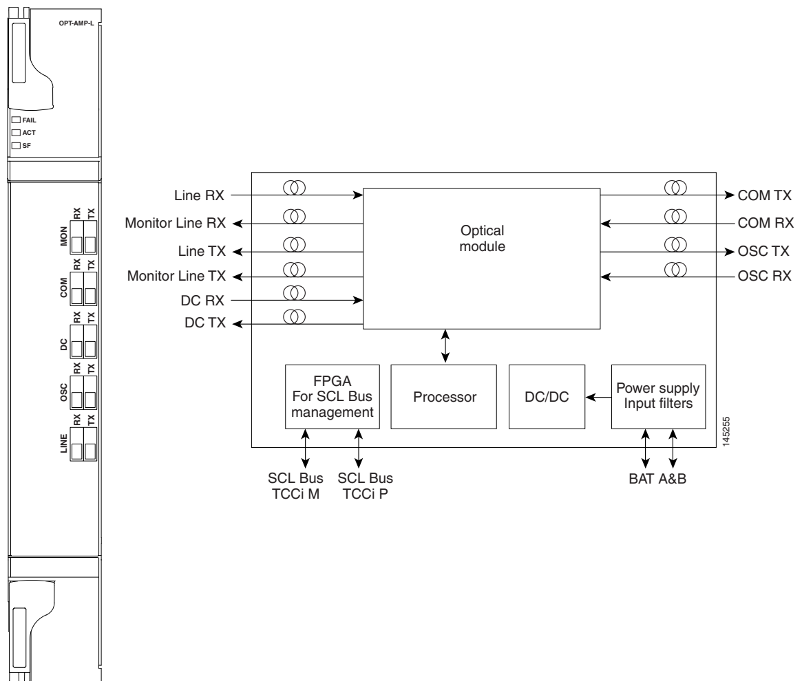
Figure 2-36 OPT-AMP-L Faceplate
