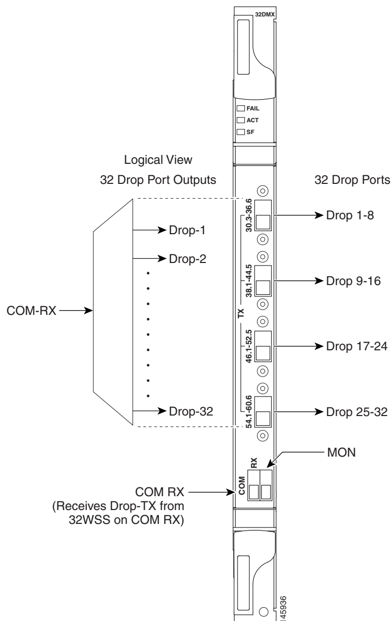
Figure 2-44 32DMX Faceplate and Ports
