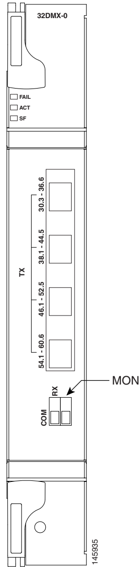
Figure 2-41 32DMX-O Faceplate
