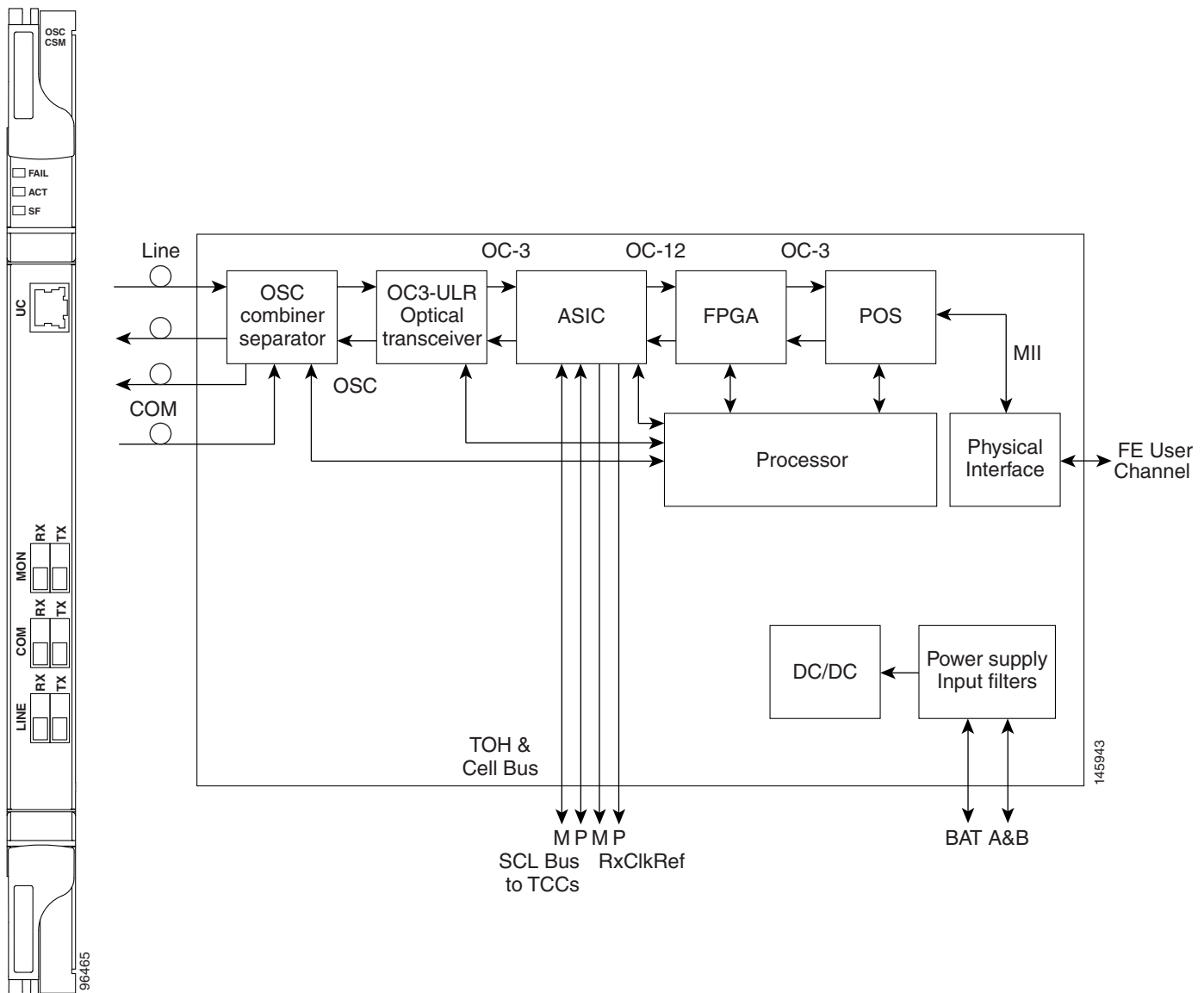
Figure 2-22 OSC-CSM Faceplate
