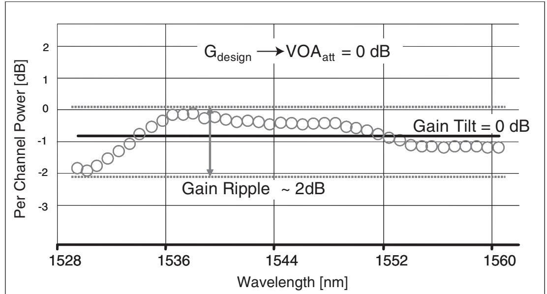
Figure 4-16 Flat Gain (Gain Tilt = 0 dB)
