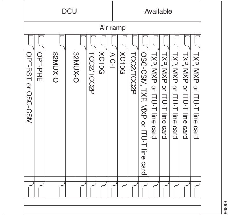
Figure 3-29 Amplified Hybrid Terminal Example
