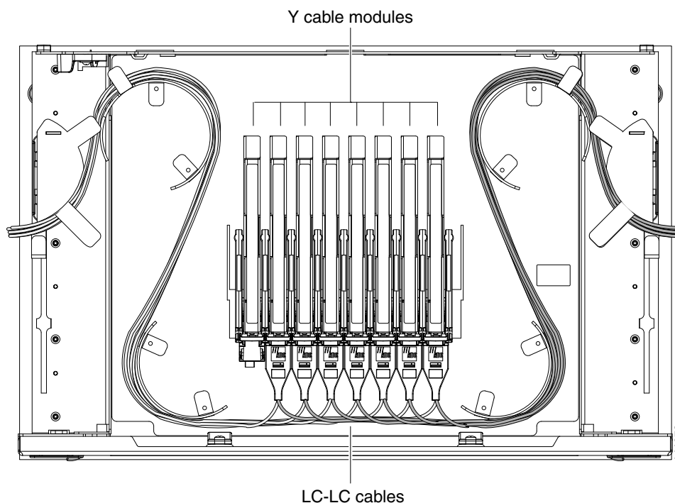
Figure 1-44 Y-Cable Module Tray
