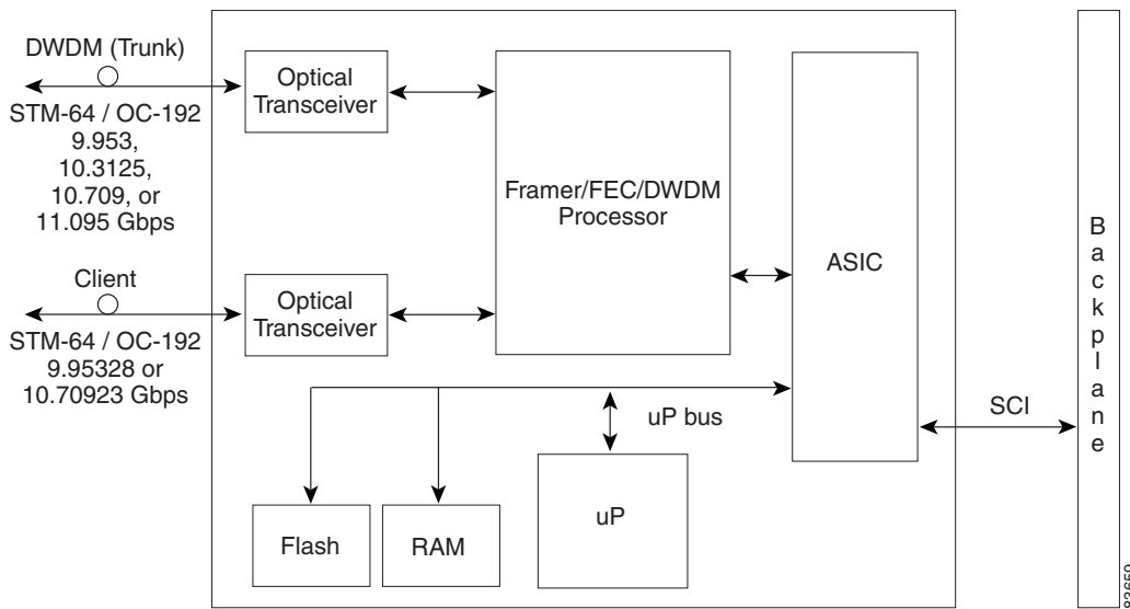
Figure 2-82 MXP_2.5G_10G Card Block Diagram
