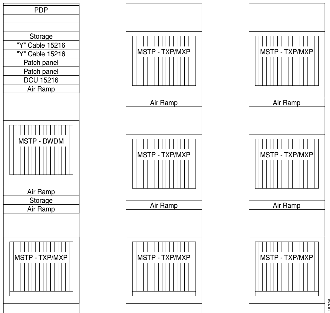
Figure 3-15 Multishelf Node Configuration
