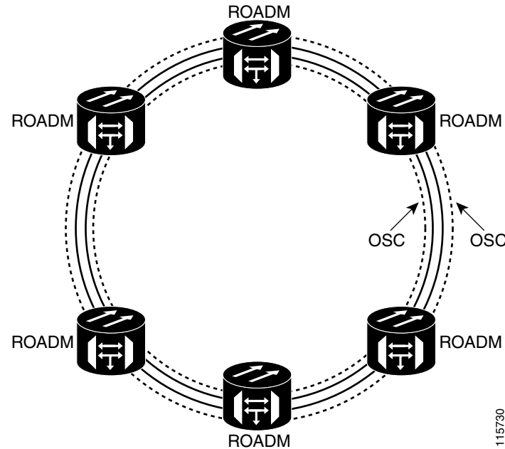
Figure 4-3 Any-to-Any Ring
