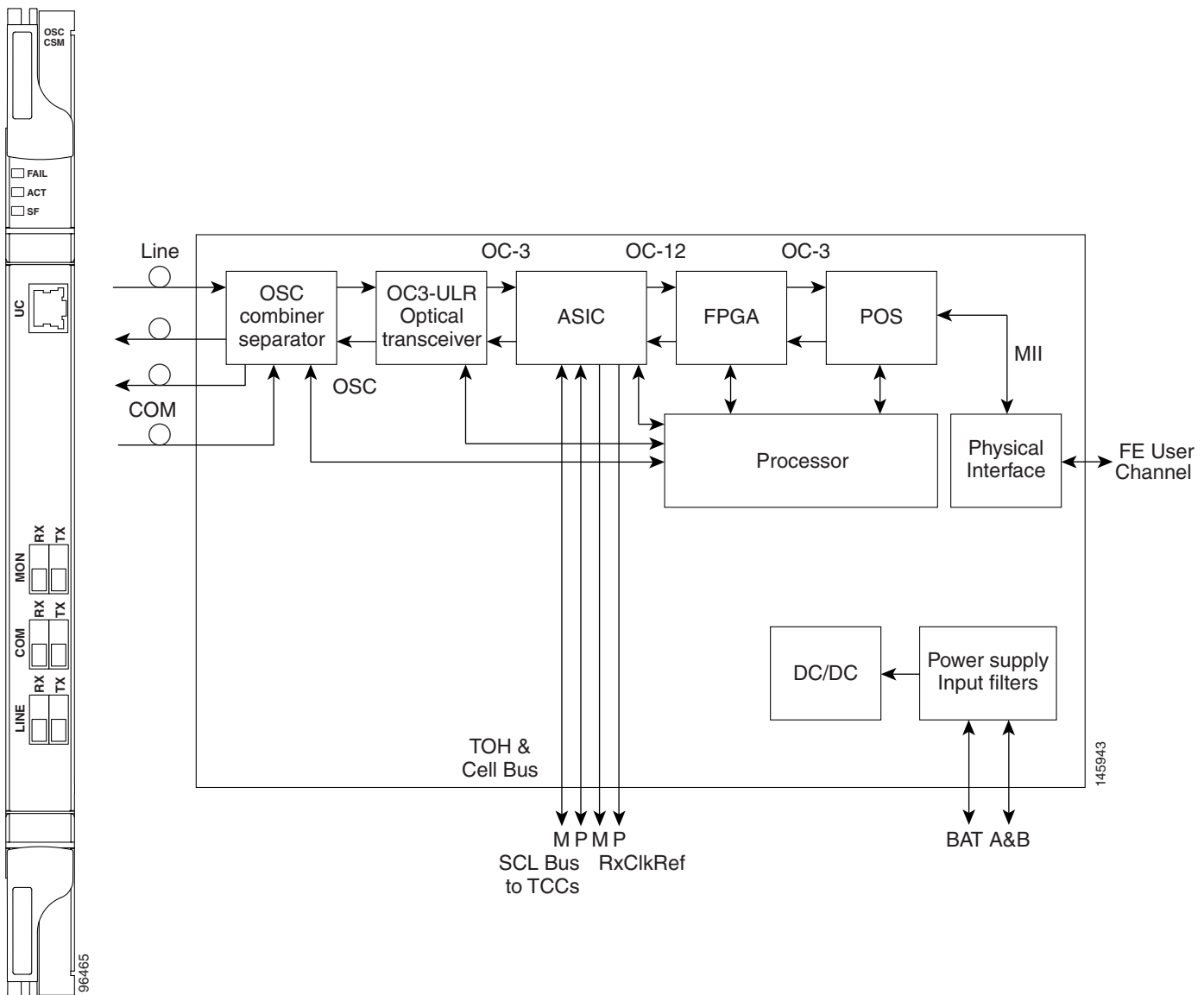
Figure 2-22 OSC-CSM Faceplate
