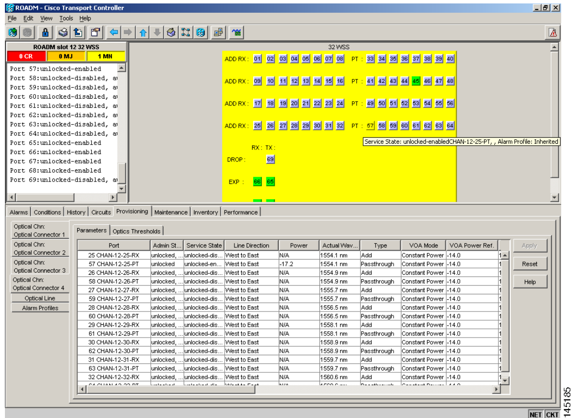
Figure 1-35 Optical Power Less than 6 dB Lower than Expected
