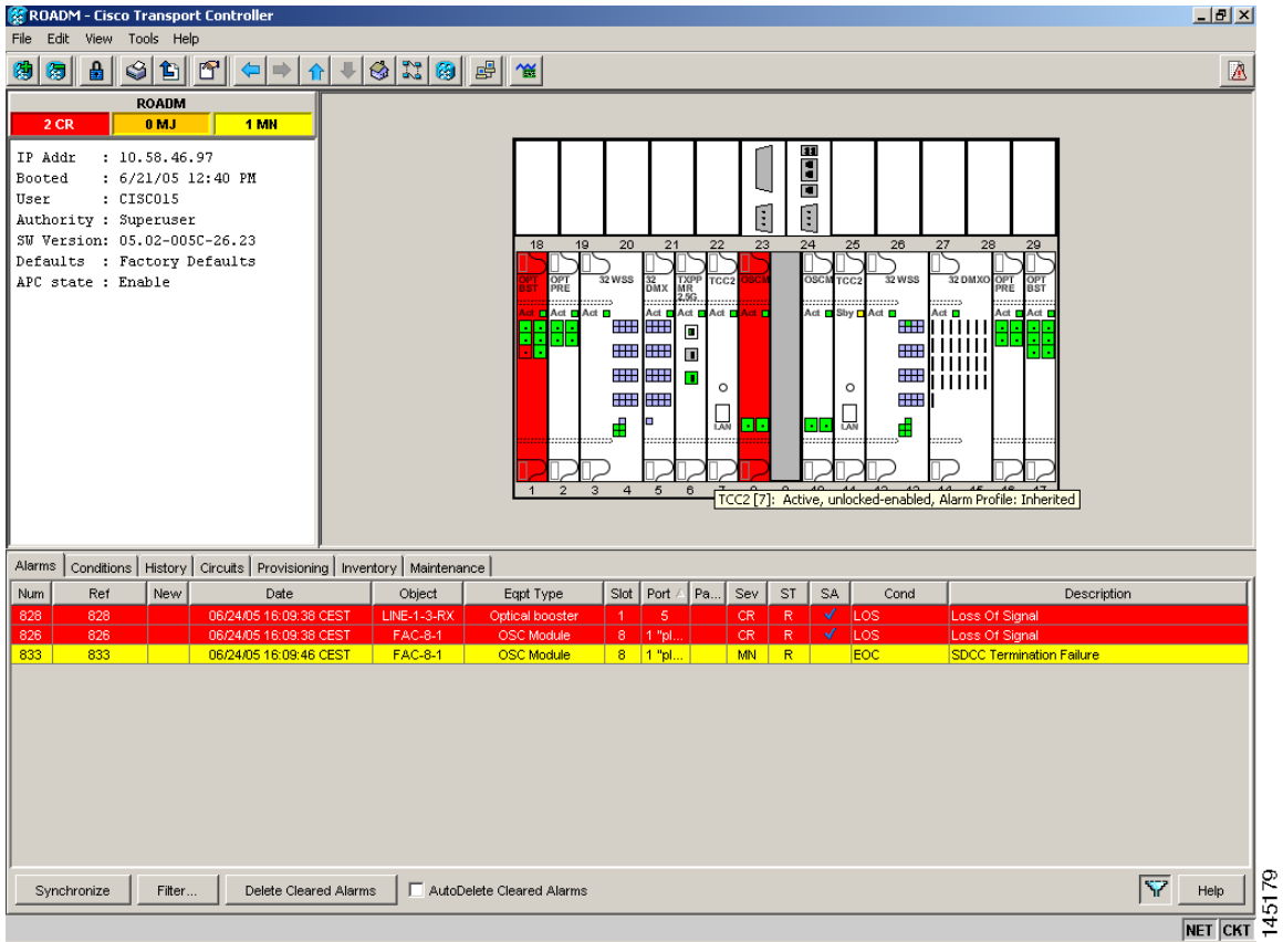
Figure 1-24 LOS Indication on the OLA Node OPT-BST
