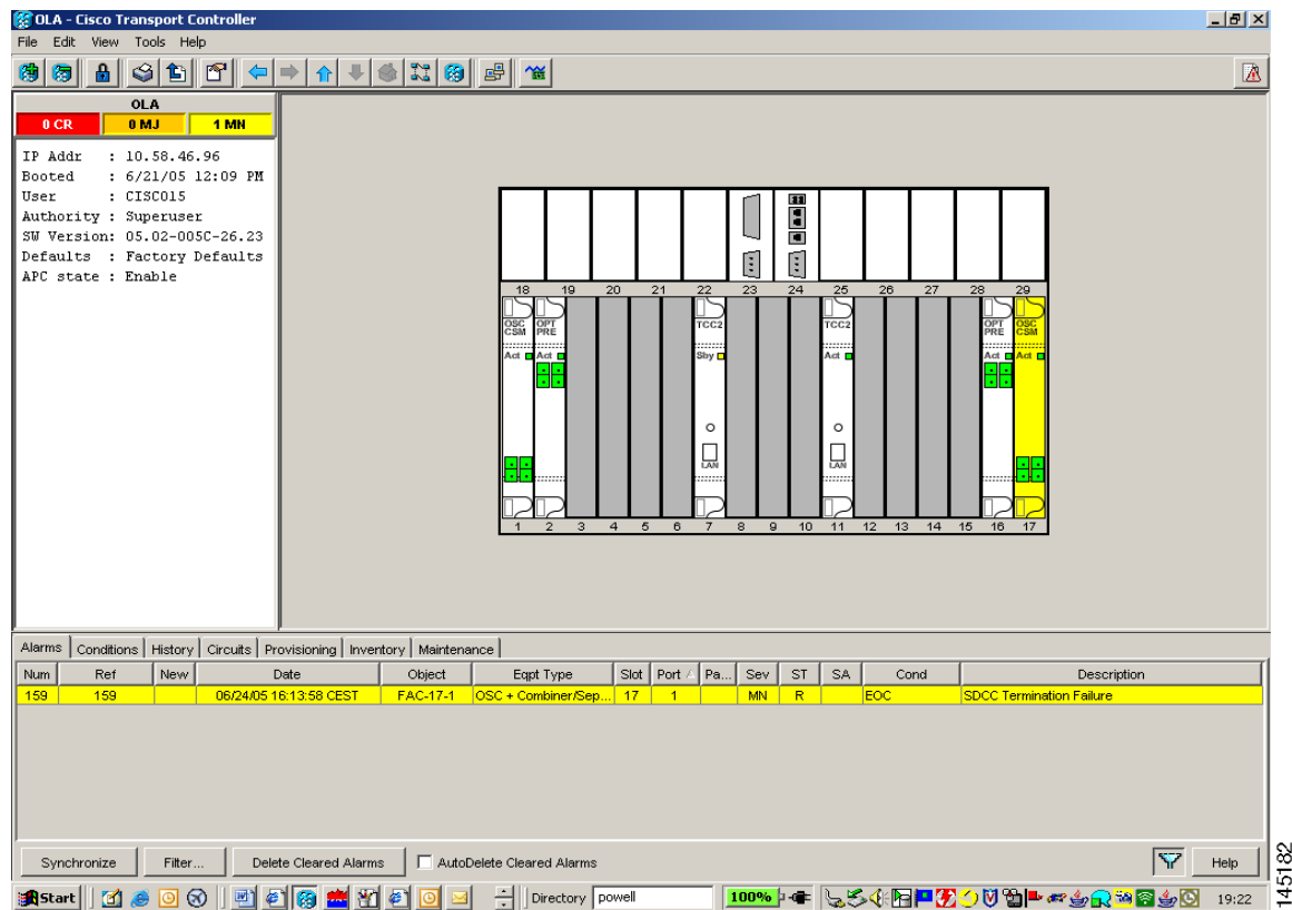
Figure 1-27 ONS 15454 SDH OLA Node View with Fault Condition for ALS MODE Disabled
