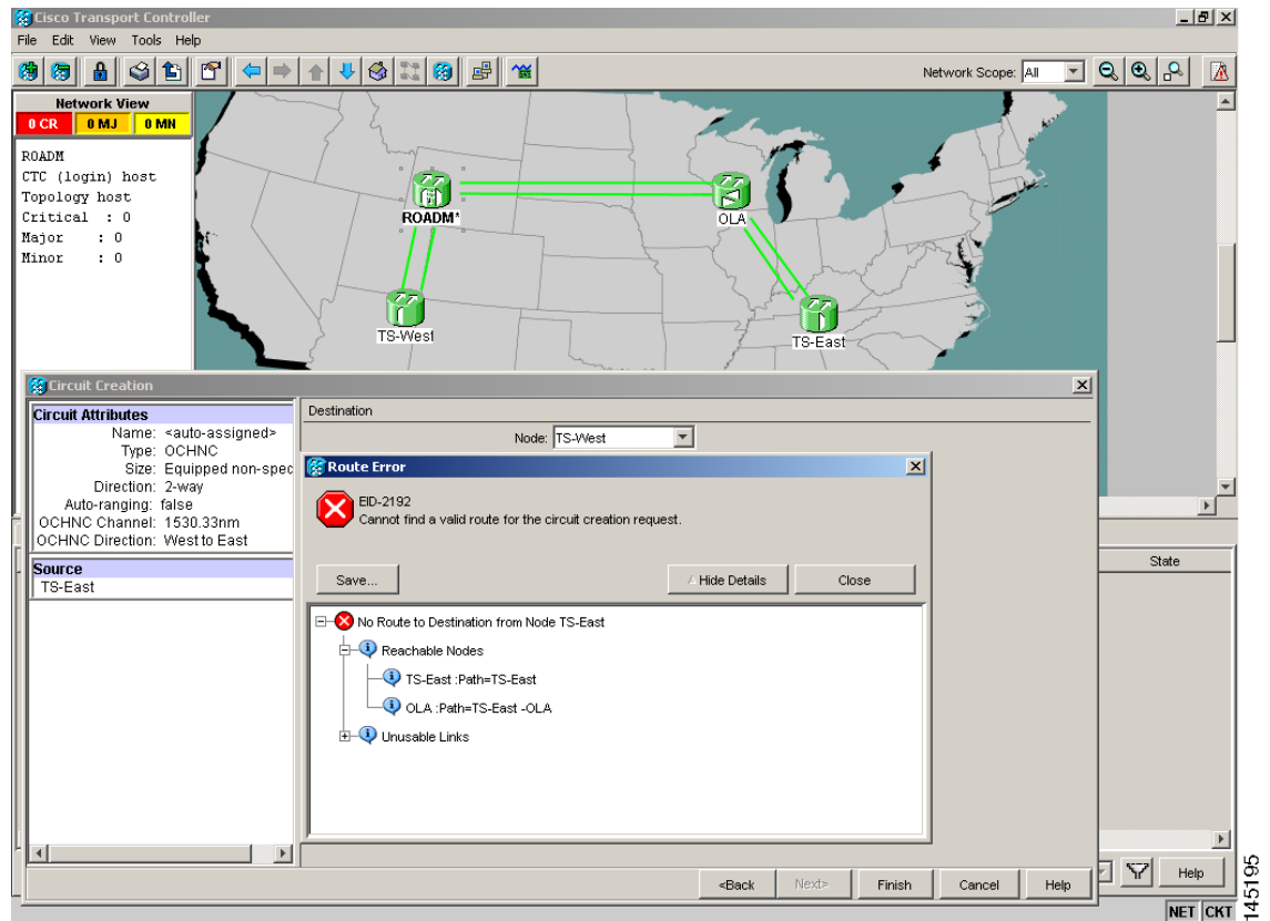
Figure 1-30 Partial Circuit
