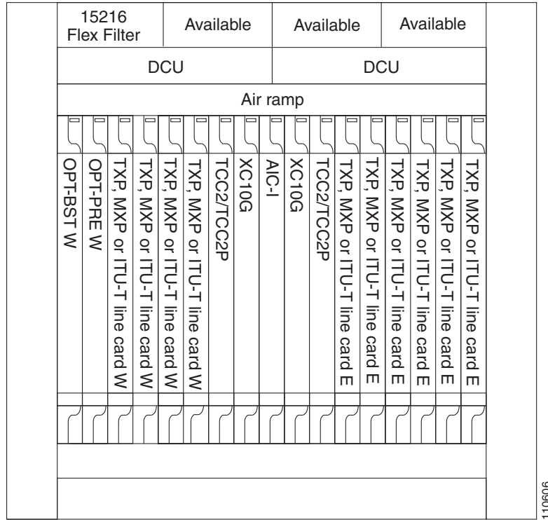
Figure 3-36 Amplified TDM Example with FlexLayer Filters
