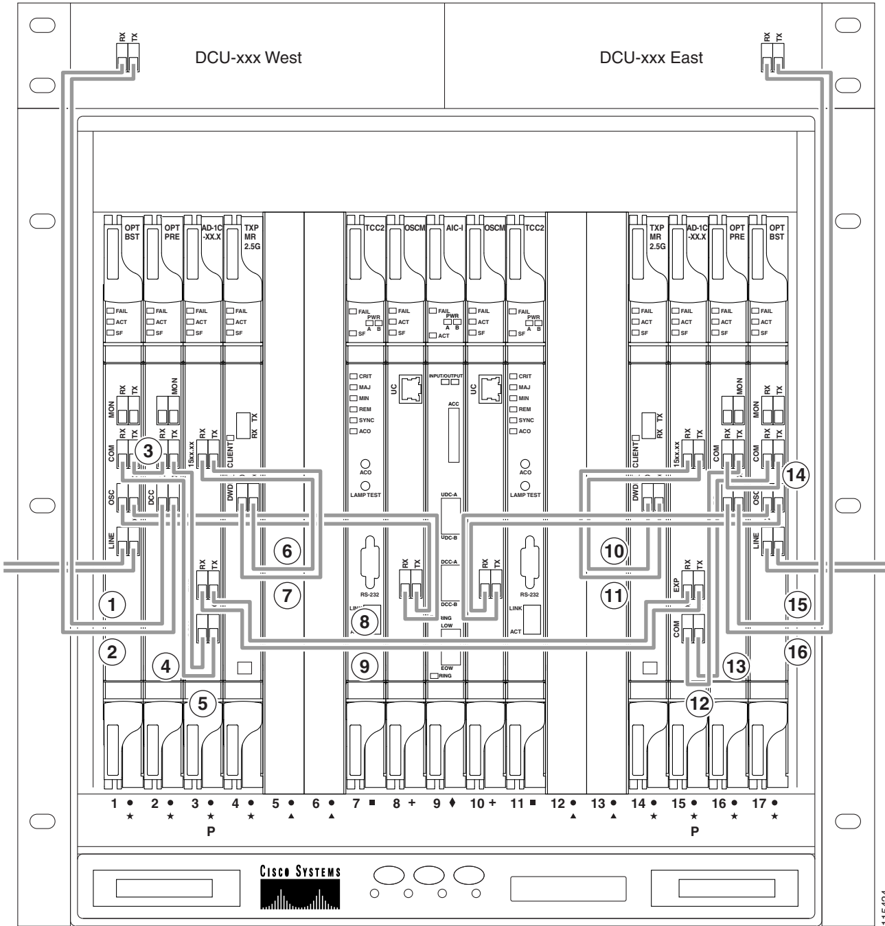
Figure 3-20 Fiberling an Amplified OADM Node
