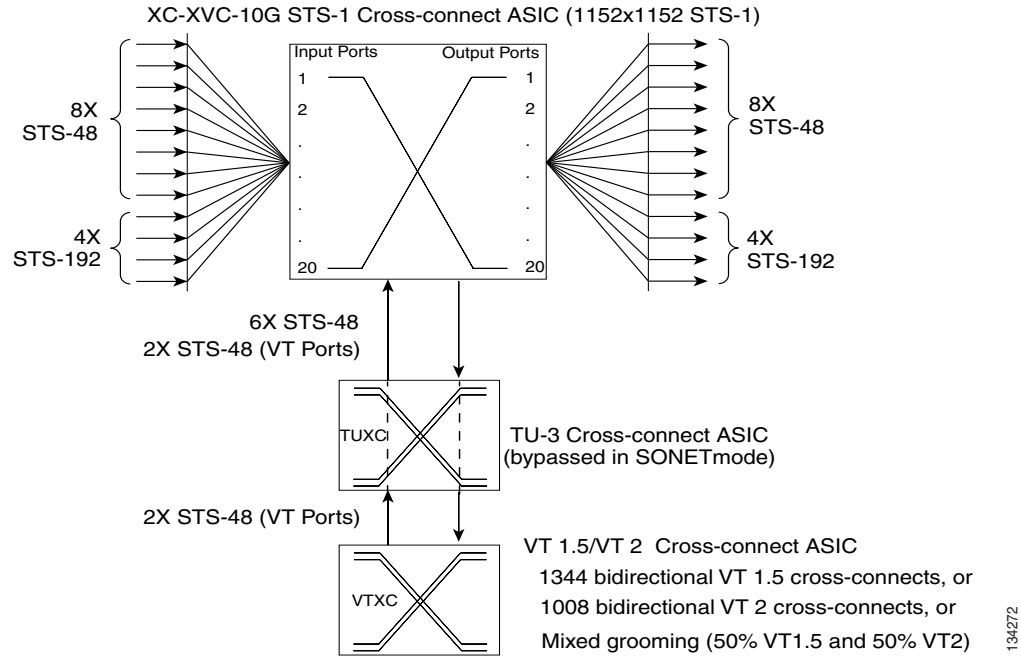
Figure 2-8 XC-VXC-10G Cross-Connect Matrix
