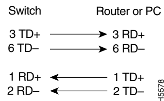
Figure 1-30 Straight-Through Cable
