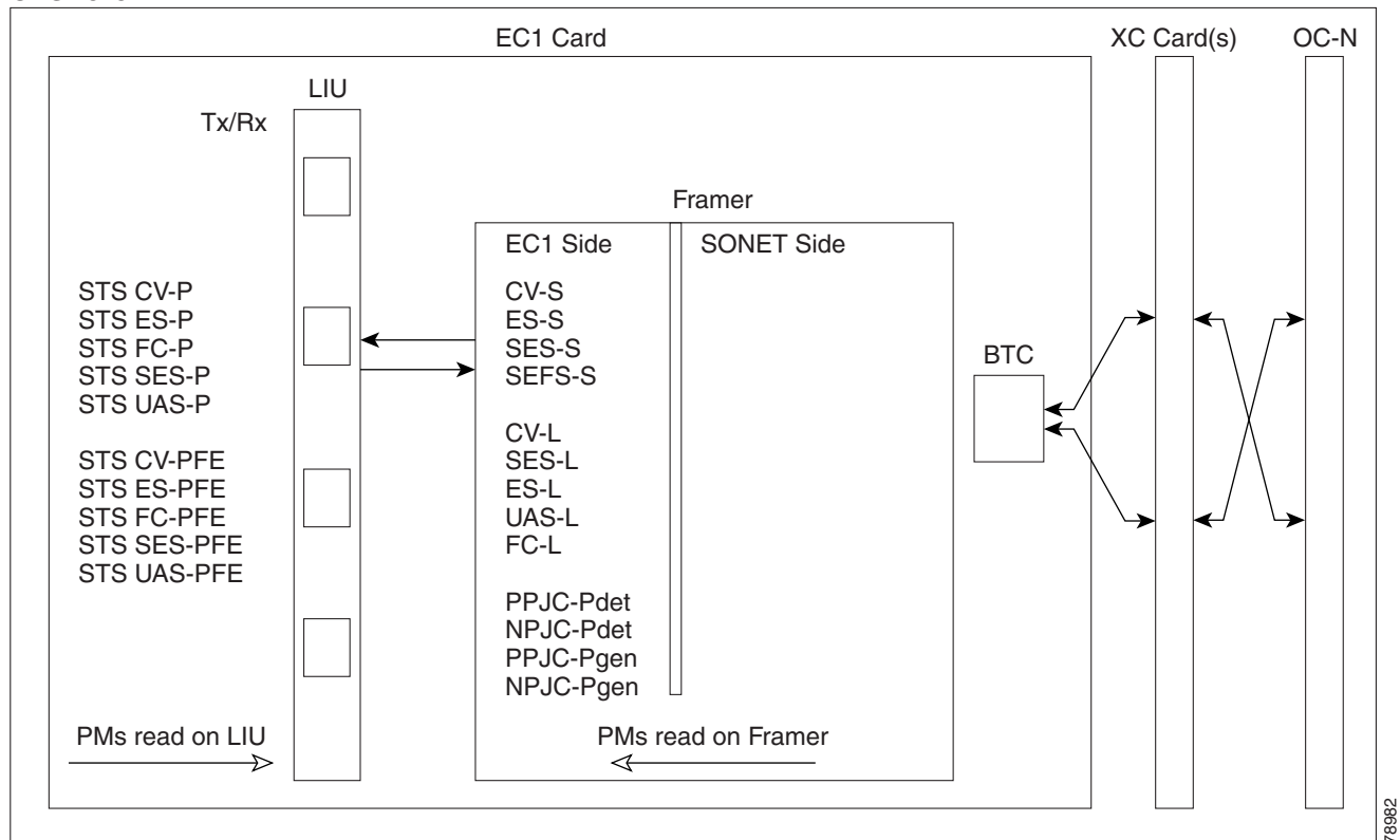
Figure 15-3 PM Read Points on the EC1-12 Card
