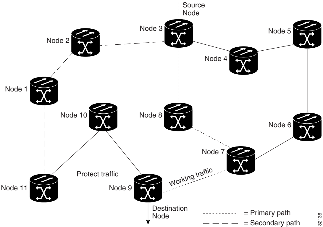
Figure 12-18 Path-Protected Mesh Network
