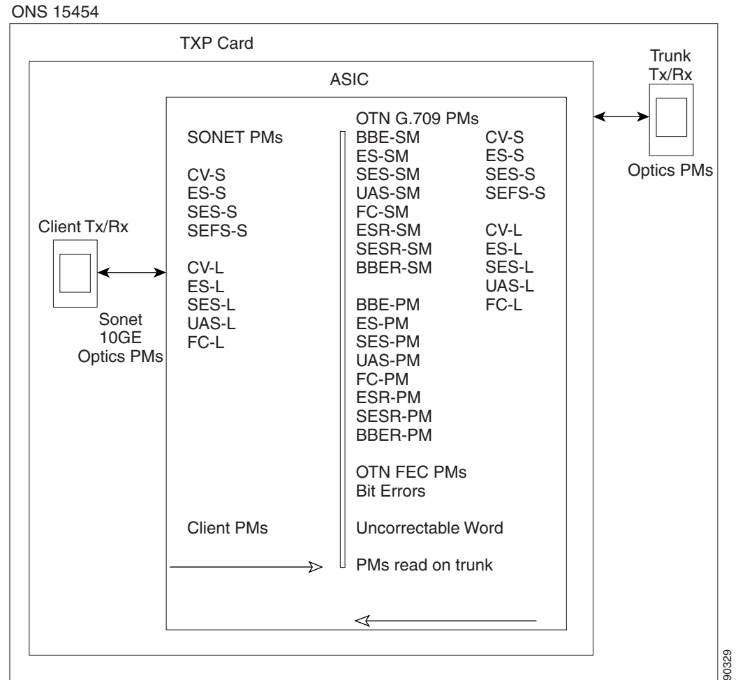
Figure 5-1 ONS 15454 ANSI Node PM Read Points for TXP_MR_10G Card
