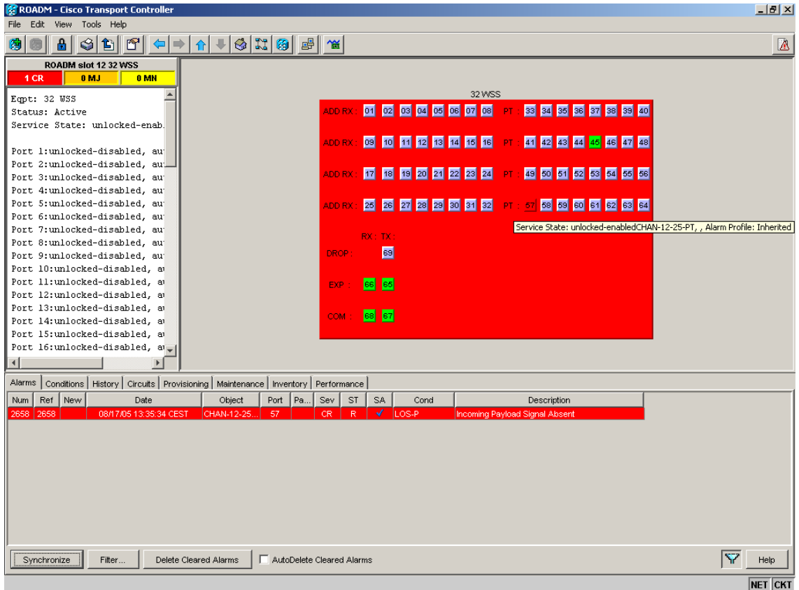
Figure 1-32 LOS-P Indication on the VOA Port
