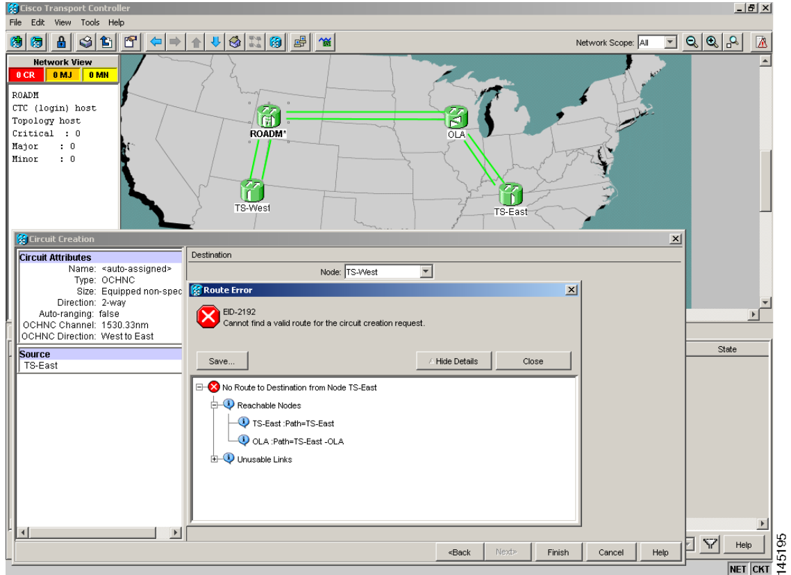
Figure 1-29 Partial Circuit
