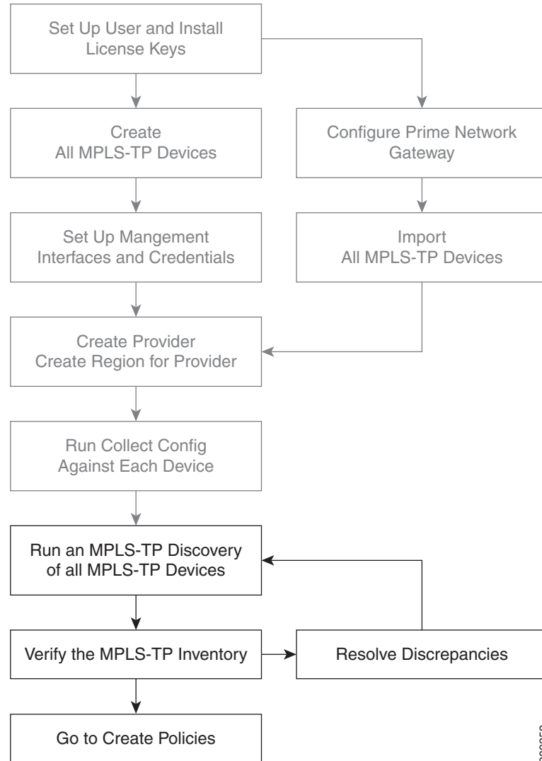
Figure 7-2 Preconfiguration Process
