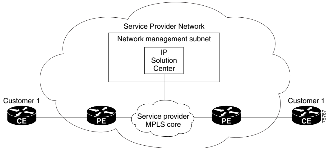
Figure 6-17 Service Provider Network and Unmanaged CEs
