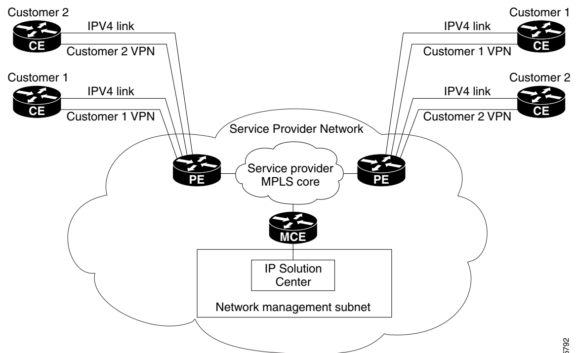
Figure 6-20 Out-of-Band Technique
