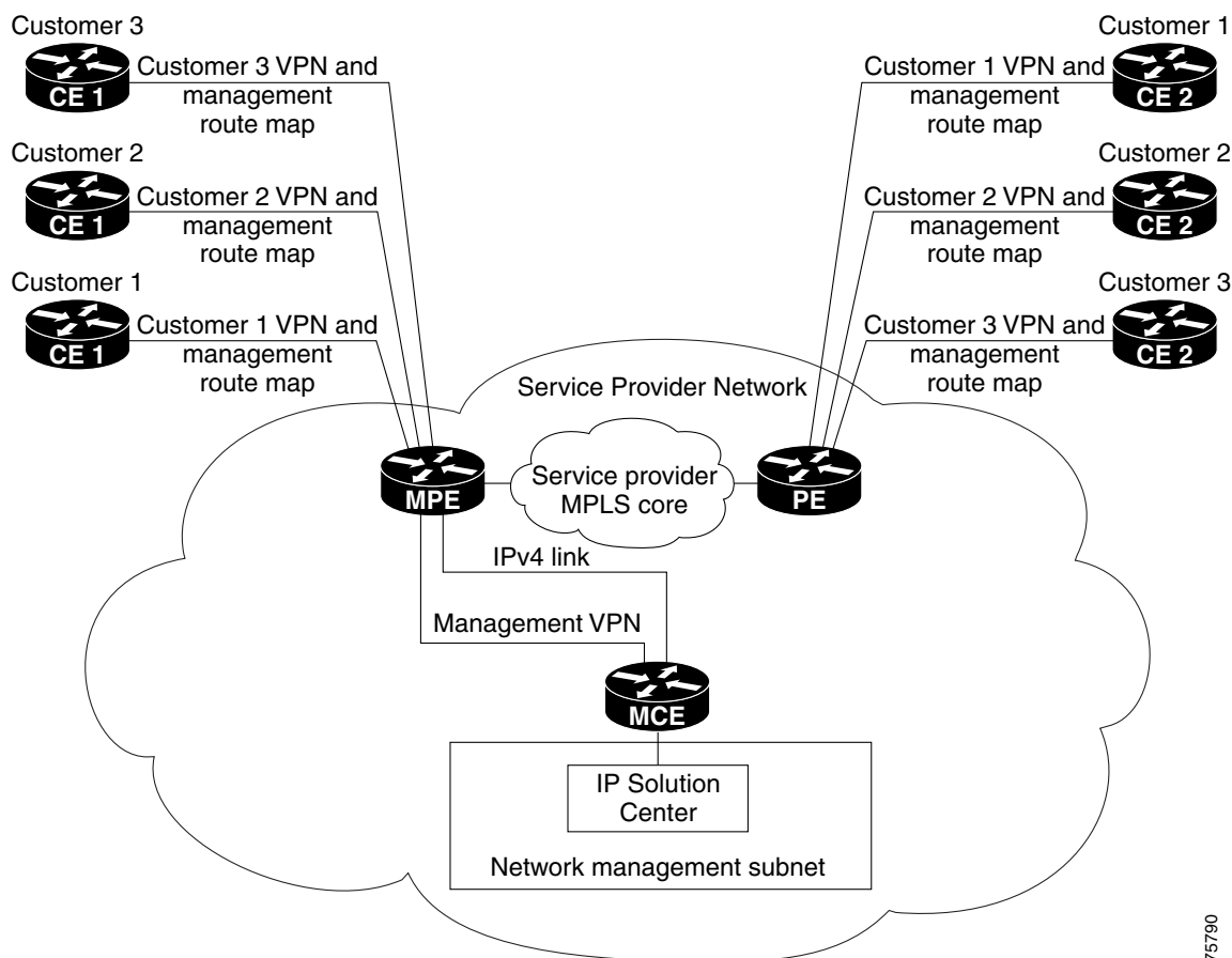
Figure 6-19 Typical Topology for a Management VPN Network
