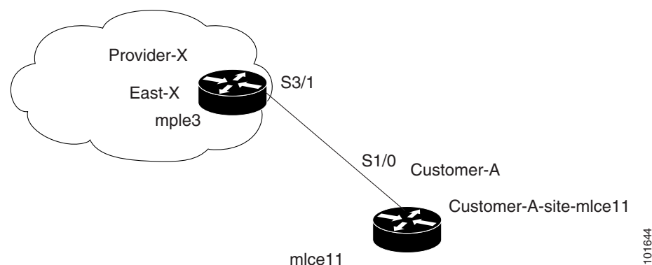
Figure 6-12 PE-CE Topology
