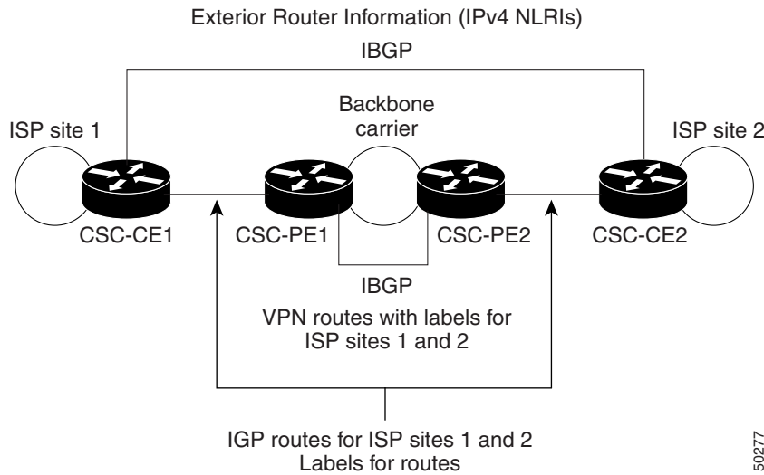
Figure 6-23 Backbone Carrier Exchanging Routing Information with a Customer Carrier Who Is an ISP
