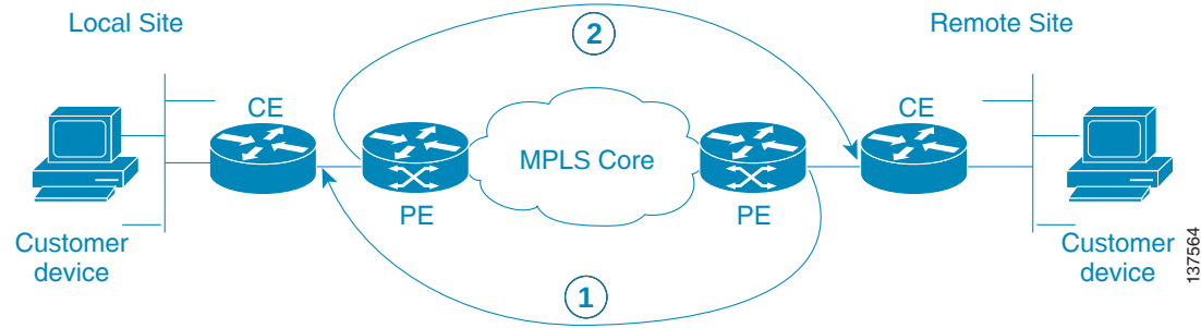
Figure 12-26 IOS VRF Ping Connectivity Tests
