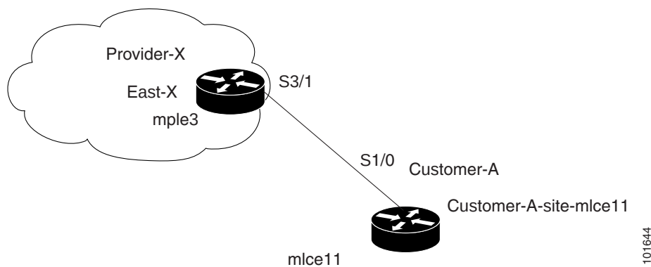
Figure 6-12 PE-CE Topology
