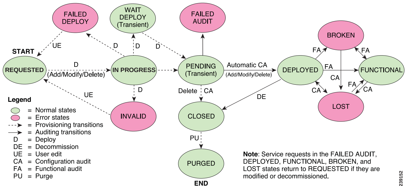
Figure 9-1 Service Requests States Transition Diagram
