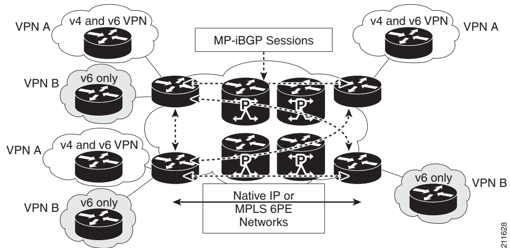
Figure 6-3 6VPE Deployment
