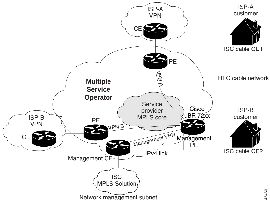
Figure 6-21 Example of an MPLS VPN Cable Network
