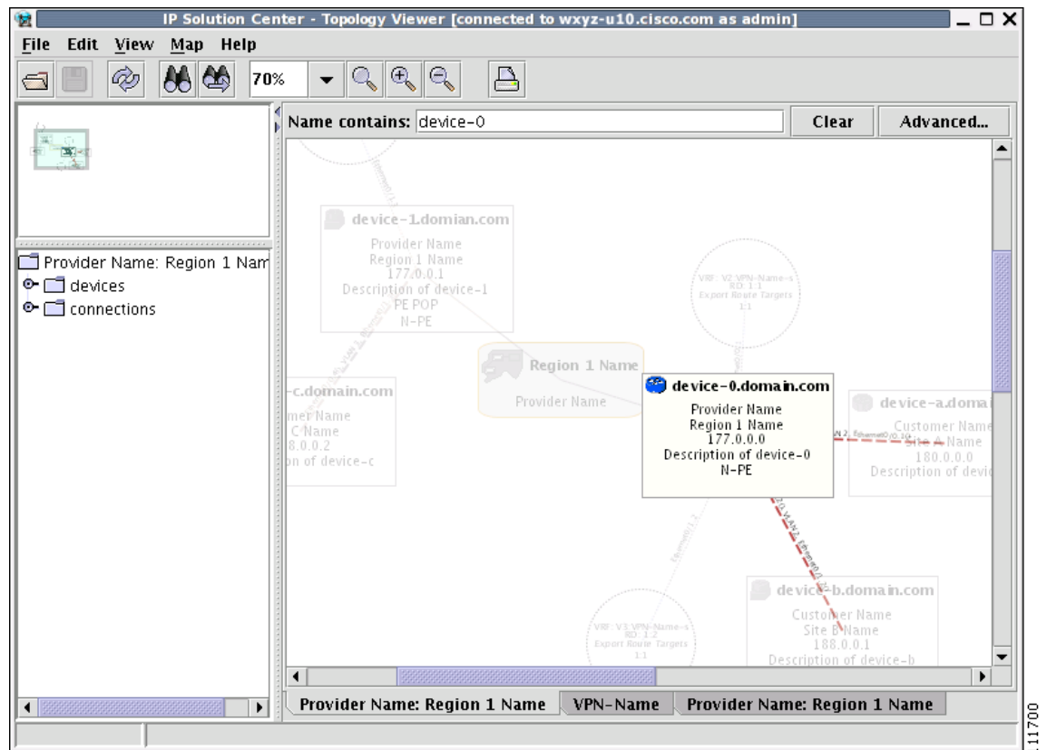
Figure 13-14 Physical View with Dimmed Nodes
