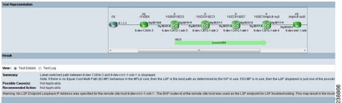
Figure 12-24 Test Results Window—LSP Visualization
