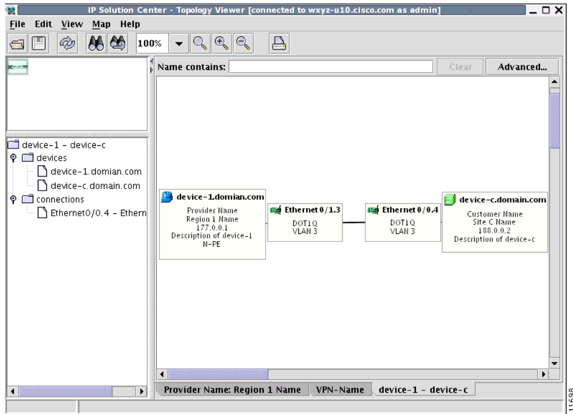
Figure 13-11 Detailed Connection View
