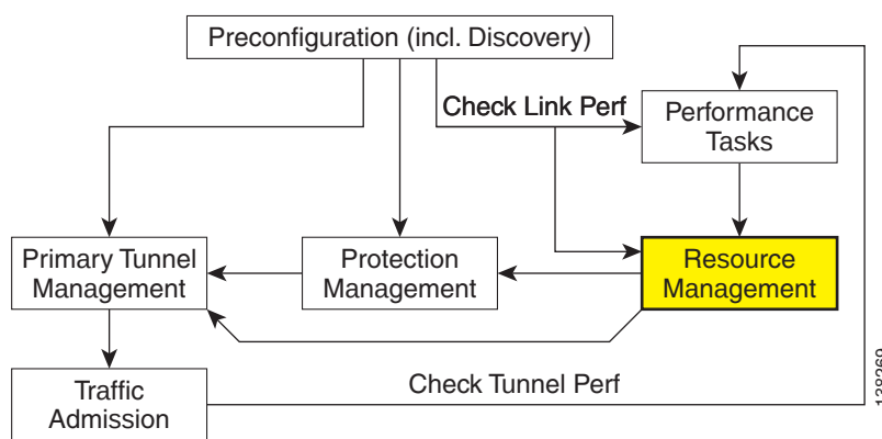
Figure 8-11 Prime Provisioning Process Diagram - Resource Management
