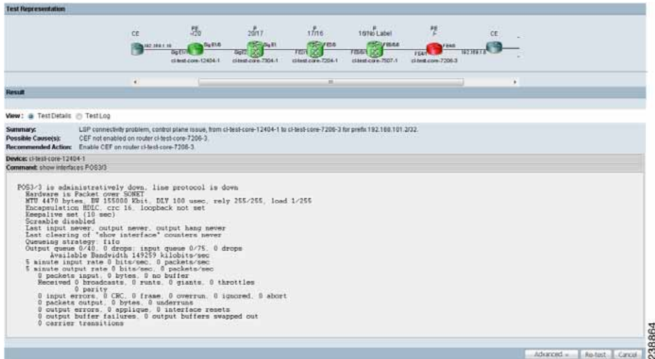
Figure 12-19 Test Results Window with Failure Specific Additional Information Displayed
