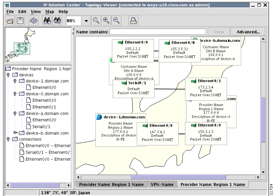
Figure 13-18 Physical View with a Map of Japan
