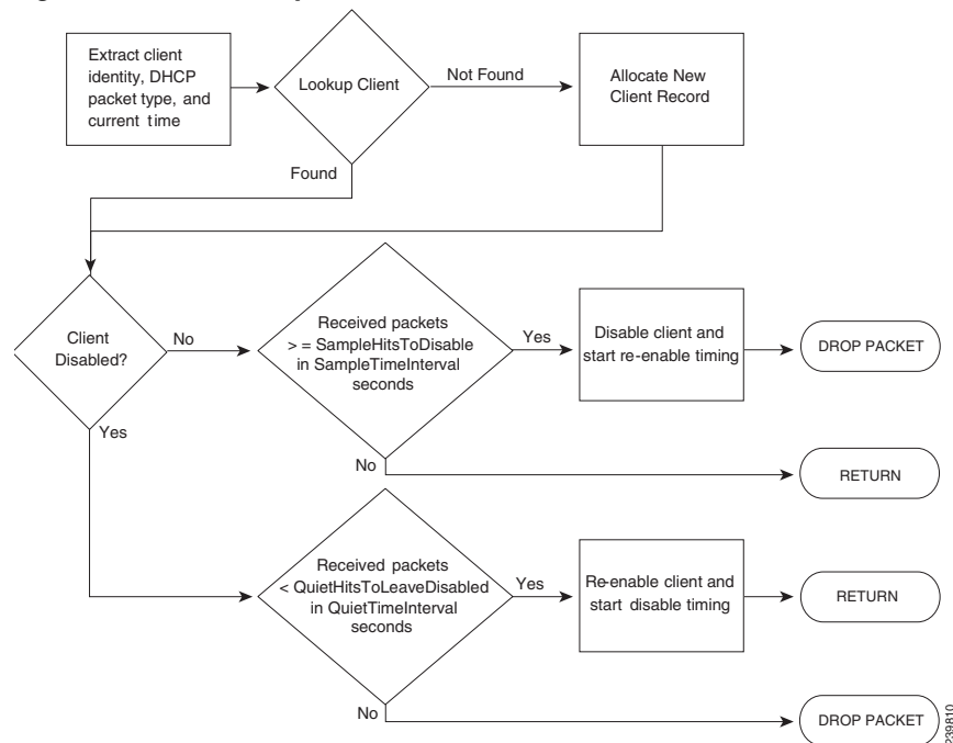
Figure 25-1 Chatty Client Filter Flow
