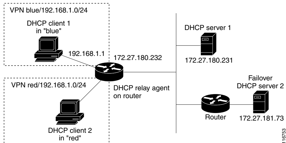
Figure 21-4 Virtual Private Network DHCP Configuration
