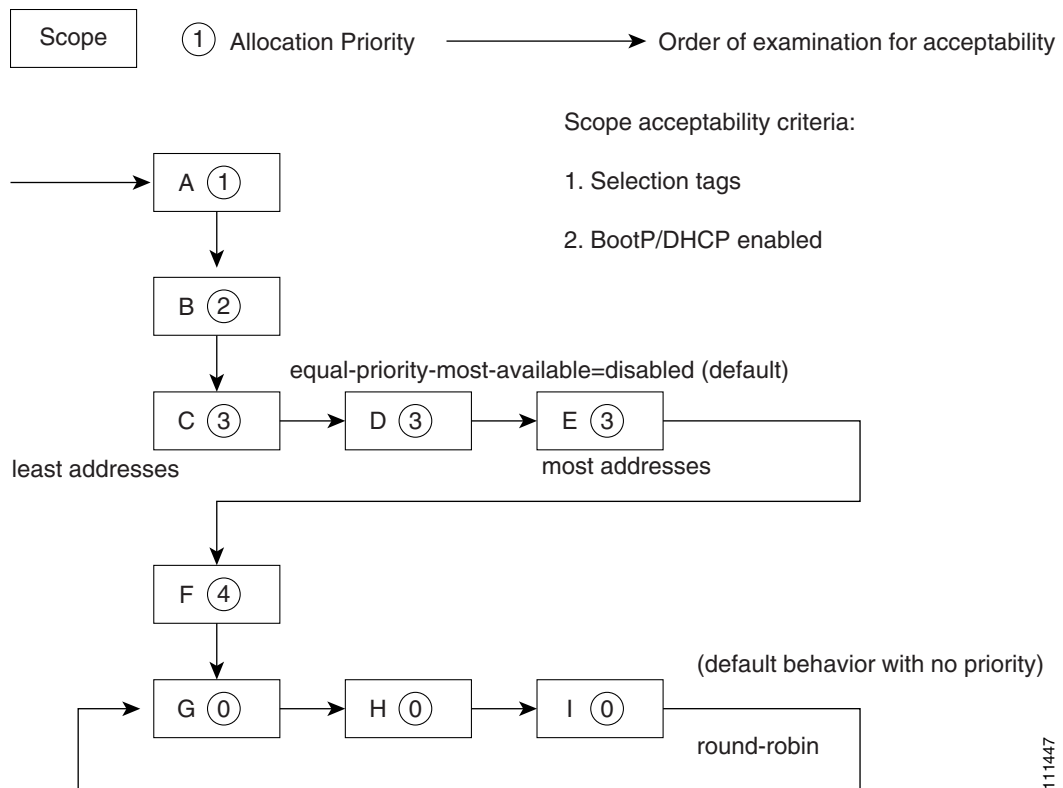
Figure 22-1 Scope Allocation Priority
