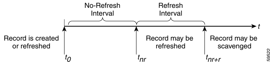
Figure 30-1 Address Record Scavenging Time Line Intervals
