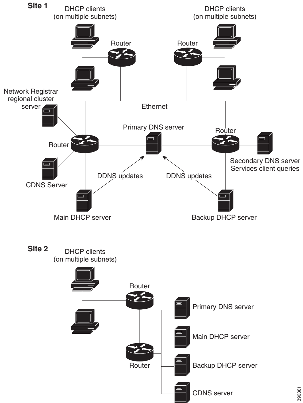
Figure 4-3 Large Enterprise or Service Provider Network Configuration
