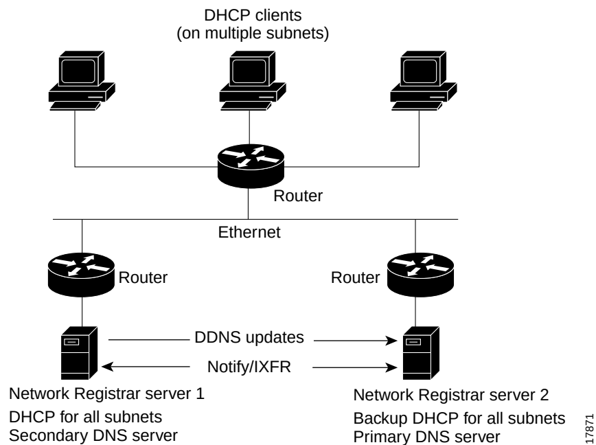
Figure 4-2 Small-to-Medium LAN Configuration
