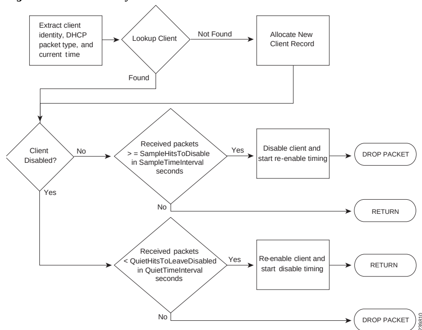
Figure 24-1 Chatty Client Filter Flow
