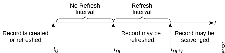
Figure 29-1 Address Record Scavenging Time Line Intervals
