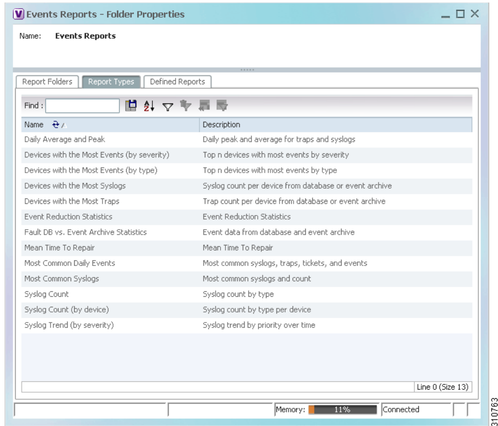
Figure 10-9 Folder Properties
