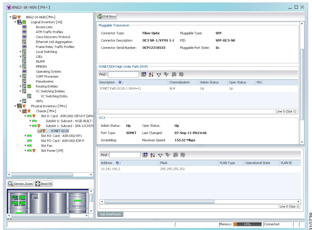
Figure 18-9 SONET/SDH Interface in Physical Inventory
