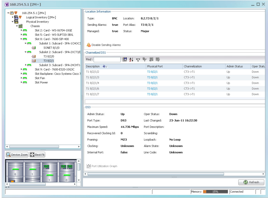
Figure 18-11 T3 DS1 Channelization Properties in Physical Inventory
