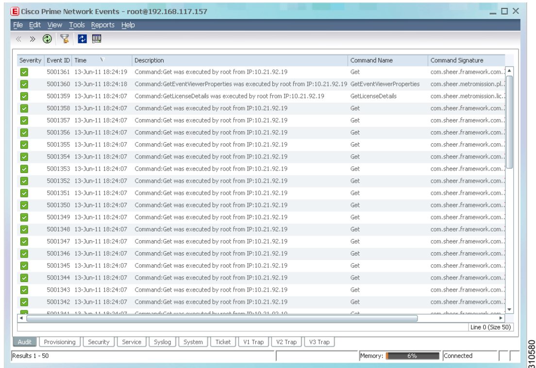
Figure 8-1 Audit Tab
