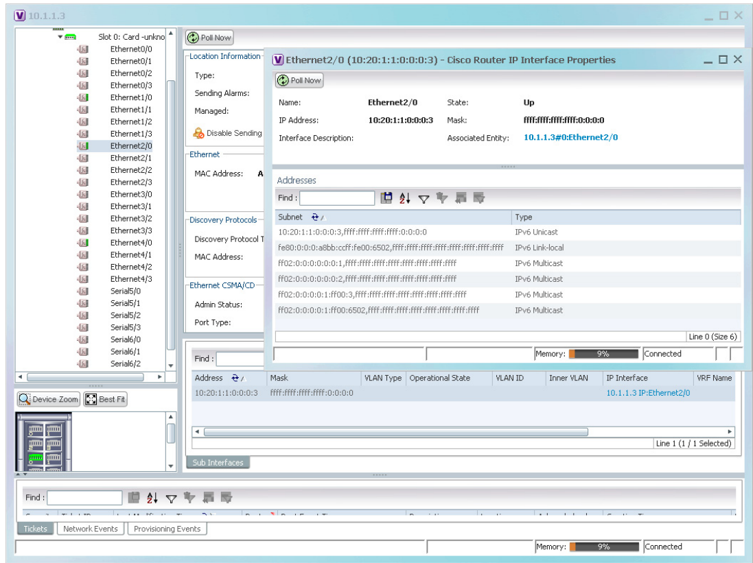
Figure 16-2 Port with IPv6 Addresses
