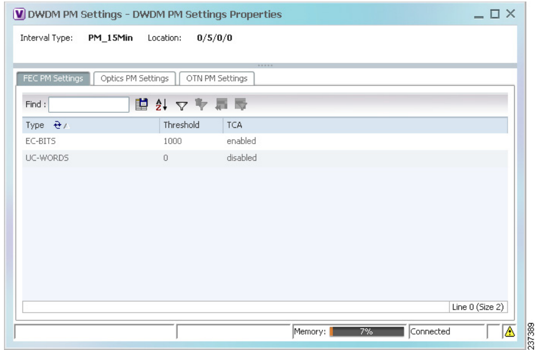
Figure 15-4 Client DWDM PM Settings Properties Window
