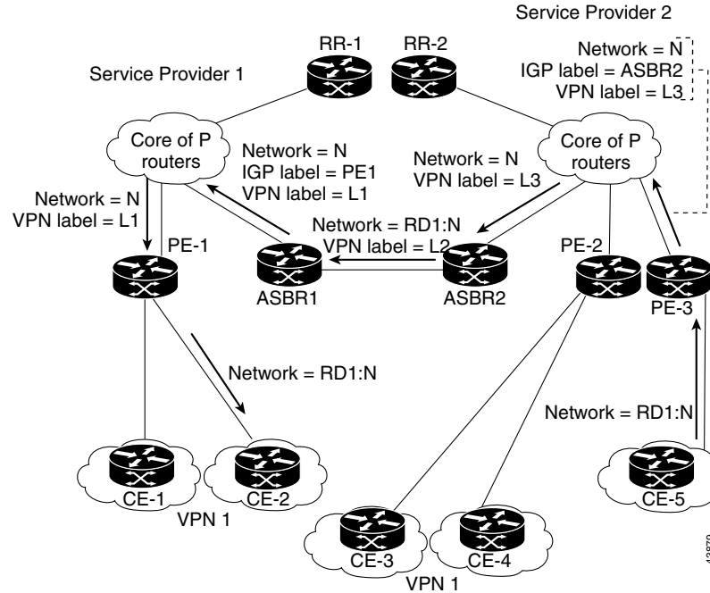
Figure 5-34 Forwarding Packets Between Two Autonomous Systems
