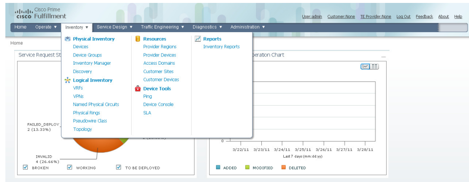
Figure 1-9 Inventory Selections
