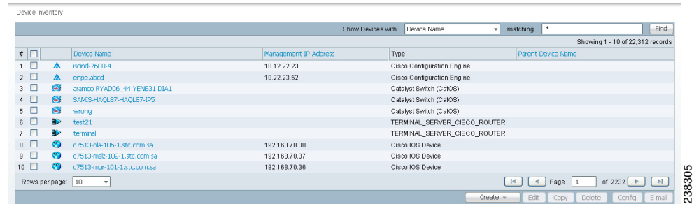
Figure 1-7 Devices—Icons
