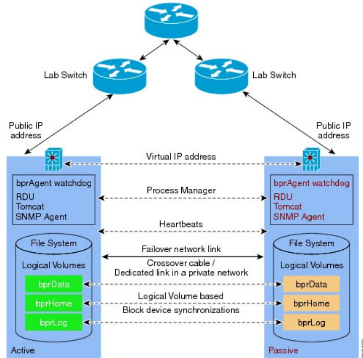
Figure 2: RDU Redundancy
