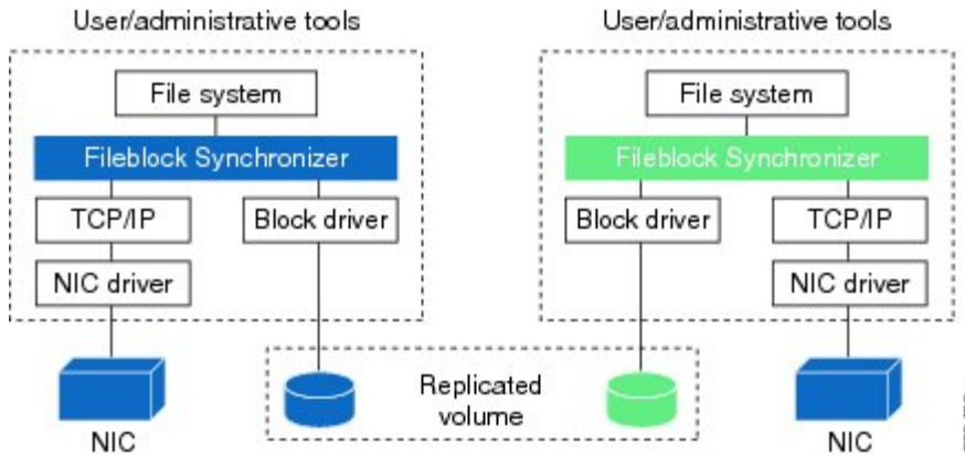
Figure 4: Database Mirroring
