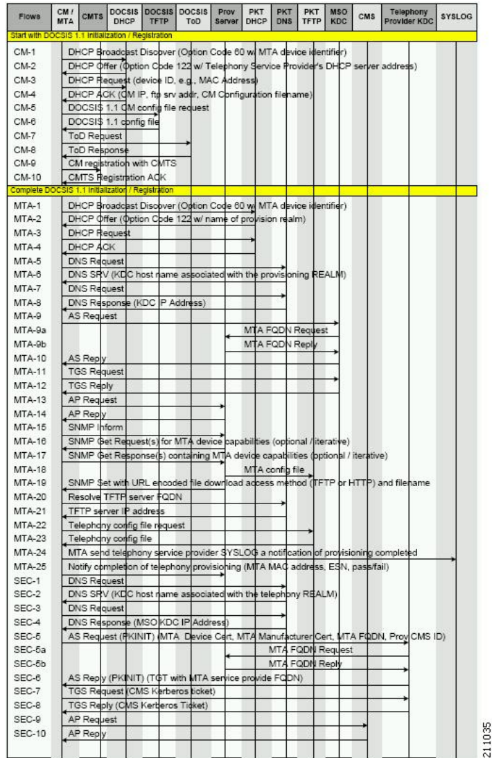
Figure 13: Embedded-MTA Secure Power-On Provisioning Flow
