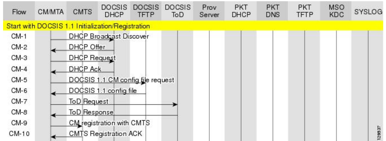
Figure 14: DOCSIS DHCPv4 Provisioning Flow
