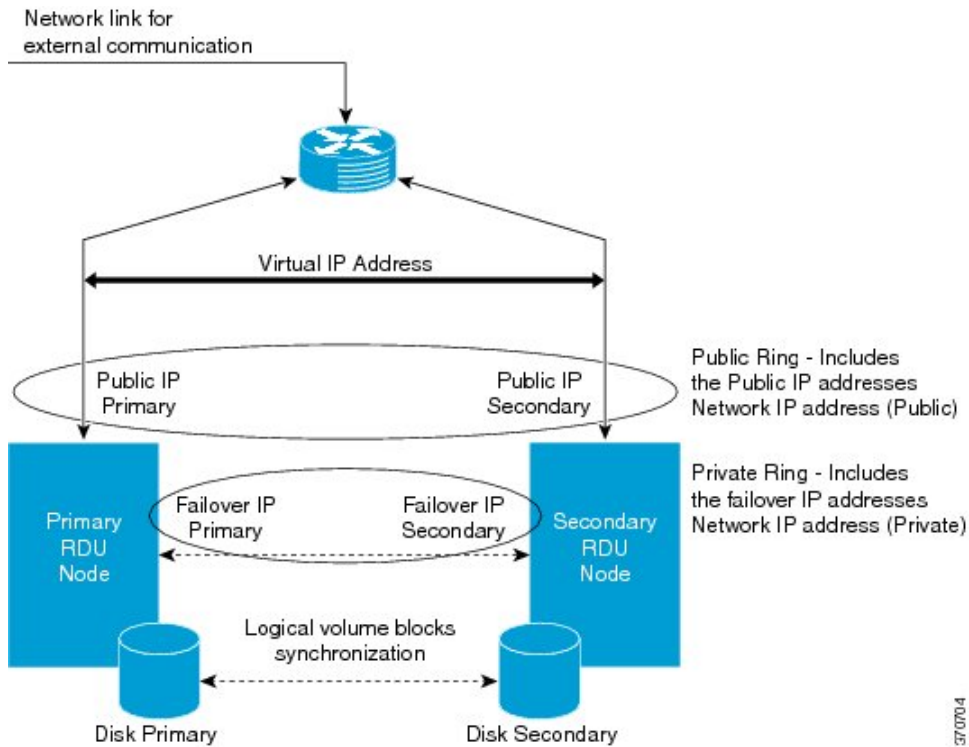
Figure 6: Dual Ring Support
