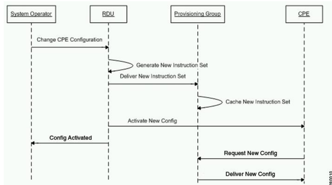
Figure 19: Workflow of Device Configuration Update
