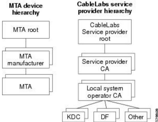
Figure 20: PacketCable Certificate Hierarchy
