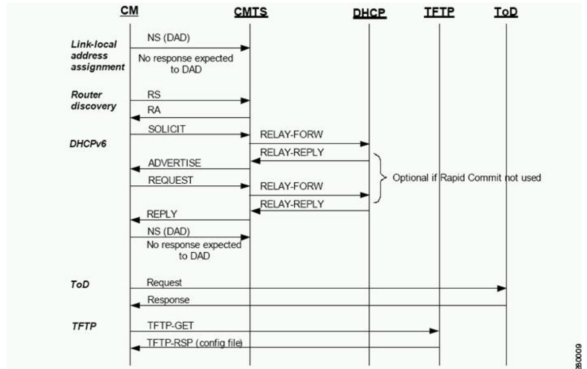
Figure 15: DOCSIS DHCPv6 Provisioning Flow
