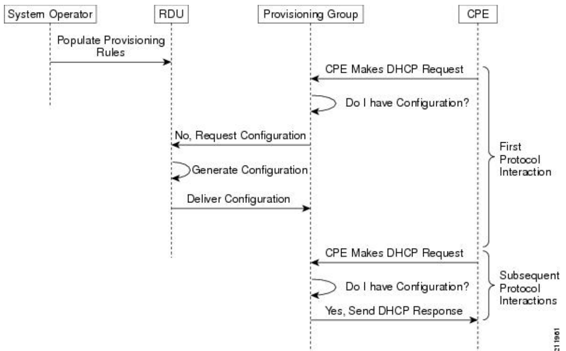
Figure 18: Workflow of Initial Device Configuration – Self-Provisioned Mode
