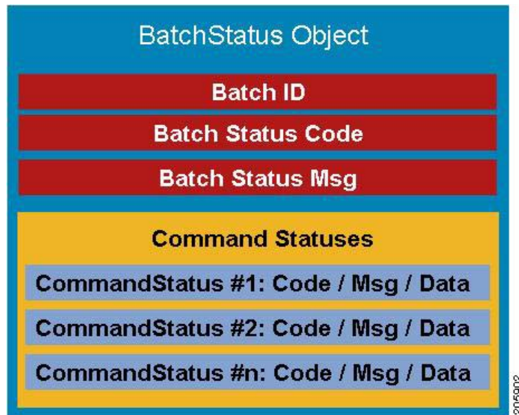
Figure 4-2 Batch Status Object
