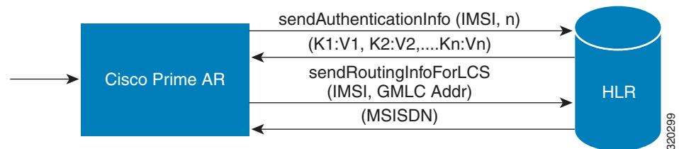
Figure 23-1 MAP Service
