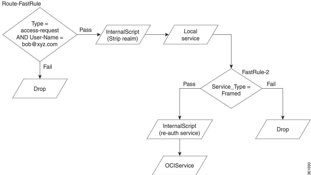
Figure 19-1 FastRules Workflow
