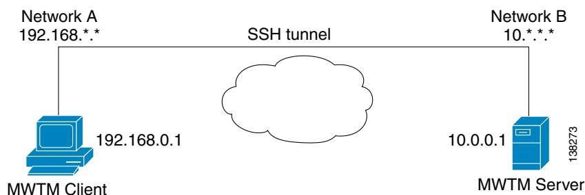
Figure H-6 Port-Forwarding Communication
